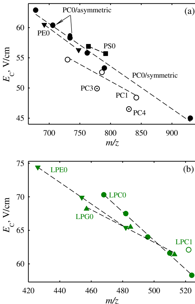
Figure 1. Measurements for phospholipids (a) and lysophospholipids (b): data (symbols) and linear regressions for categories with at least two points (lines). Filled symbols are for saturated lipids, empty symbols are for unsaturated ones, and the number after lipid classification indicates the degree of unsaturation
