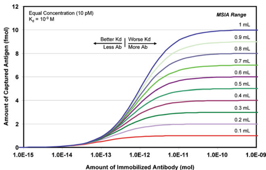
Figure 1. Binding curves derived for an analyte at a constant concentration of 10 pM, and varying volumes of samples. The X-axis is the amount of antibody immobilized to a stationary phase (in moles) and incubated with the sample volume (in mL). The Y-axis is the amount of analyte captured at equilibrium (in fmol). The affinity constant for the system is constant for all curves ( K_d=10^{-9} M), as would be employed in a real situation. However, all curves will shift systematically as indicated with the use of an alternate antibody. In the ideal situation, all components of the analytical system (antibody load and K_d , sample volume, analyte concentration and the lower limit of detection of the mass spectrometer) are in alignment to perform the concerted analytical technique known as mass spectrometric immunoassay
