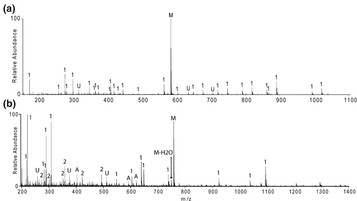
Figure 1. QTOF MS 2 spectra for Peptides A and B in the 2+ charge state, at m/z (a) 584 and m/z (b) 758. Each “1” refers to a single cleavage, “2” refers to a double cleavage, “U” refers to an unknown ion, and “A” refers to an ambiguous assignment. Some assignment labels have been omitted due to space constraints
