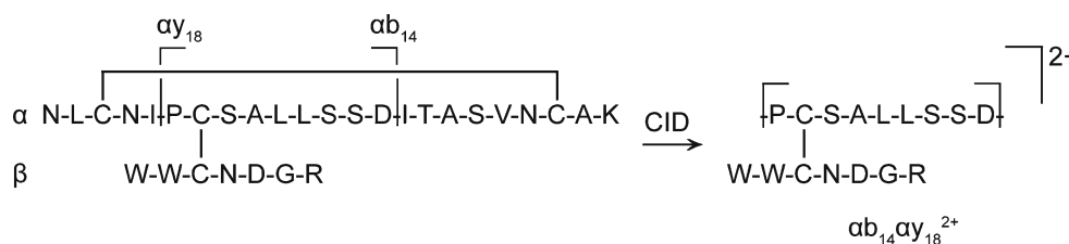
Figure 3. Inter-peptide disulfide bond can be assigned as the center cysteine residue due to this peak corresponding to a double cleavage product at m/z 904.33
