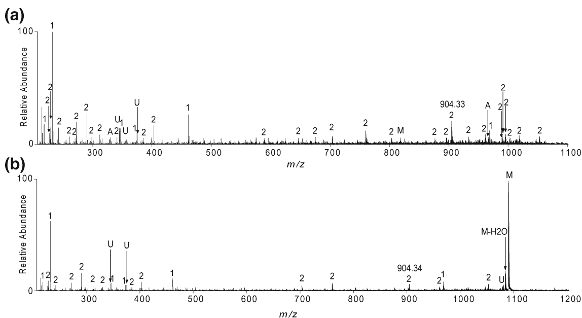
Figure 2. (a) QTOF MS 2 spectrum for Peptide D in the 4+ charge state at m/z 817. Each “1” refers to a single cleavage and “2” refers to a double cleavage. (b) QTOF MS 2 spectrum for Peptide D at m/z 1090, an ion in the 3+ charge state. Each “1” refers to a single cleavage, “2” refers to a double cleavage, “U” refers to an unknown ion, and “A” refers to an ambiguous assignment. Some assignment labels have been omitted due to space constraints
