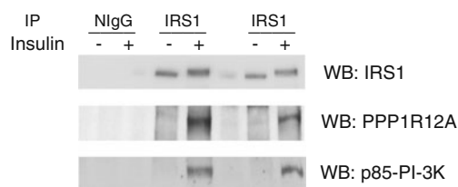
Figure 3. PPP1R12A and the p85 regulatory subunit of PI 3-K interact with IRS-1. L6 myotubes were serum-starved for 4 h and either left untreated or stimulated with insulin (100 nM) for 15 min at 37 °C. One mg of lysate proteins were immunoprecipitated with normal IgG or IRS-1 antibodies and Western blotted with antibodies specific to either IRS-1, PPP1R12A, or p85; each graph is representative of data obtained from three independent experiments
