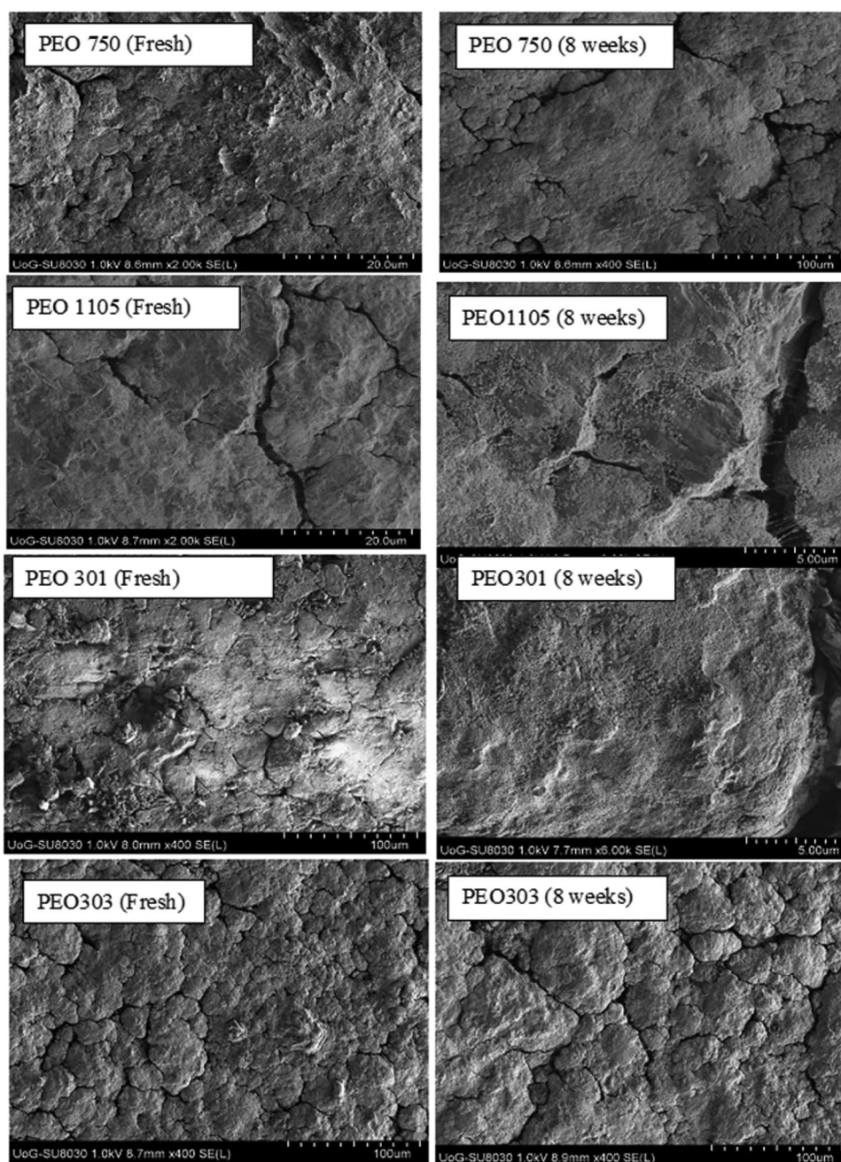
Fig. 6 SEM of various molecular weight PEOs at zero and week 8 storage times that were obtained at 25 °C
