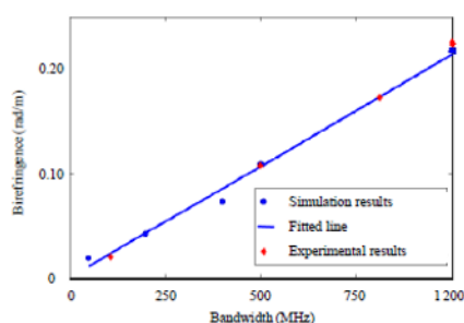
Fig. 8 Demodulated birefringence of simulation and experiments.
