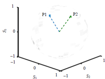
Fig. 4 Two launched lights' SOPs in the Poincaré sphere with an angular difference of 48°.
