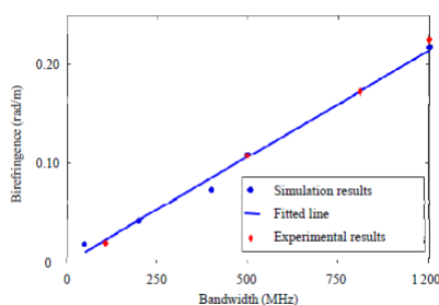
Fig. 8 Demodulated birefringence of simulation and experiments.
