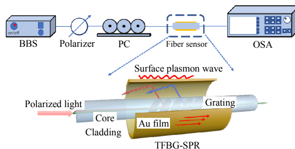
Fig. 1 Schematic illustration of experimental setup for \text{Hg}^{2+} detection.
