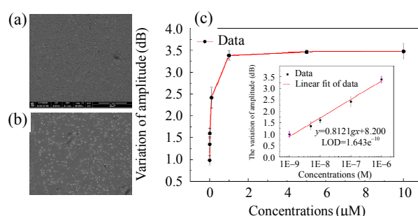
Fig. 3 Detection of mercury ions at different concentrations: (a) SEM images of physical adsorption on the sensing surface, (b) SEM images of AuNPs on the sensing surface after reaction with \text{Hg}^{2+} ions at the 100 nM concentration, and (c) spectral amplitude change and sensor detection limit as the concentration of mercury ions changes.
