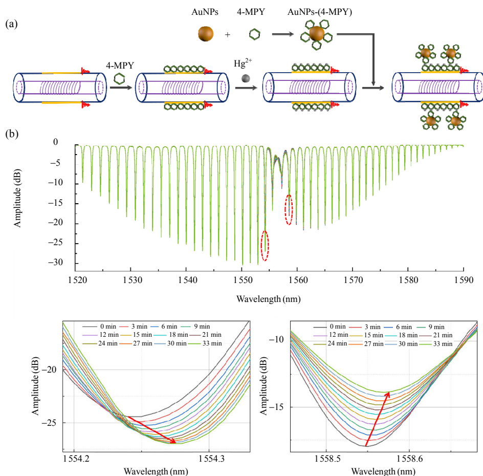
Fig. 2 Self-assembly of 4-MPY on the sensing surface and \text{Hg}^{2+} specific identification procedure: (a) schematic diagram of the TFBG-SPR sensing system for detecting mercury ions and (b) spectral response of the TFBG-SPR high order cladding mode.
