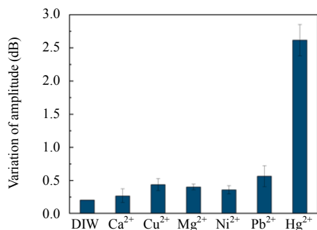
Fig. 4 TFBG-SPR biosensor selectivity for mercury ion detection (all concentrations of \text{Hg}^{2+} , \text{Ca}^{2+} , \text{Cu}^{2+} , \text{Mg}^{2+} , \text{Ni}^{2+} , and \text{Pb}^{2+} are 100 nM).
