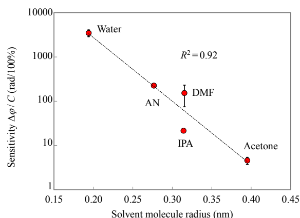
Fig. 6 Sensitivity of MZI waveguide sensor to vapor of different organic solvents as a function of solvent molecule radius. PMMA + DMABI-Ph6 cladding thickness is 1.2 \mu\text{m} .
