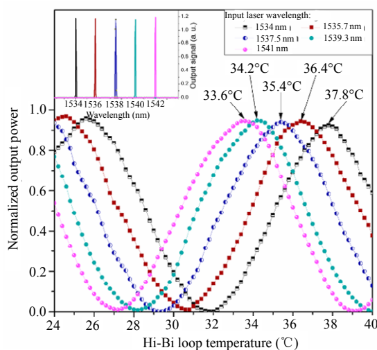
Fig. 3 HBFLM transmitted power for different input laser wavelengths on HBF temperature scanning.
