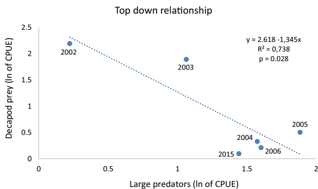
Fig. 5 Relationship between the relative abundance of decapod prey species in relation to large predators (sum of lobster, cod and poor cod, i.e. species known to feed on crustaceans) in the NTAR during the years 2002–2006 and 2015. The equation shows results from a linear regression analysis ( df = 1, 4 ) on \ln(x + 1) transformed CPUE data (catch per unit effort)
