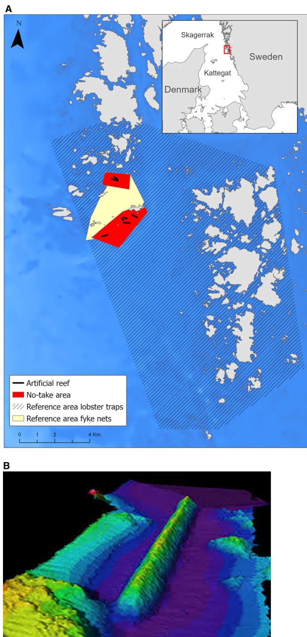
Fig. 1 A The NTAR represented by red polygons at Vinga outside Gothenburg, Sweden. The black bolded lines represent the locations of artificial reefs. The yellow polygon represents the location of fyke net sampling stations. Fyke net stations outside the NTAR (the red polygons) constitute the reference, located in the area open to fishing. For the targeted lobster sampling, reference data were additionally collected from a geographically more widespread area by collaboration with local fishers (the striped polygon). B A three-dimensional multibeam sonar image of reef 1A-1 Buskär at roughly 26–28 m depth. This reef is 350 m long, 45 m wide and 14 m high (above bottom) with its highest point 13.5 m below the surface. The image is reproduced with permission from the Swedish Maritime Association
