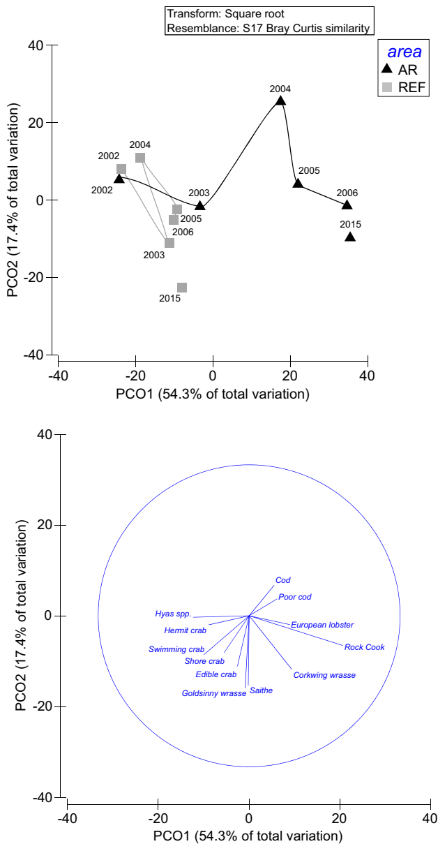
Fig. 3 Results from PCO analysis showing similarity in species composition between the NTAR (AR in the figure) and the reference area (REF in the figure) during 2002–2006 and in 2015 (above) together with vector overlays demonstrating species responsible for differences (below). Similarity was quantified by the Bray–Curtis index on square-root transformed data. The NTAR was established in 2003
