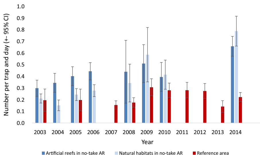
Fig. 2 Number of lobster per trap and day (CPUE) at the artificial reefs (dark blue) and at the natural lobster habitats (light blue) within the NTAR in 2003–2006, 2008–2010 and 2014, and in the reference area until 2014 (red). Error bars show \pm 95% confidence intervals. Note that the zeros for different years in the table represent missing data and not zero-catches
