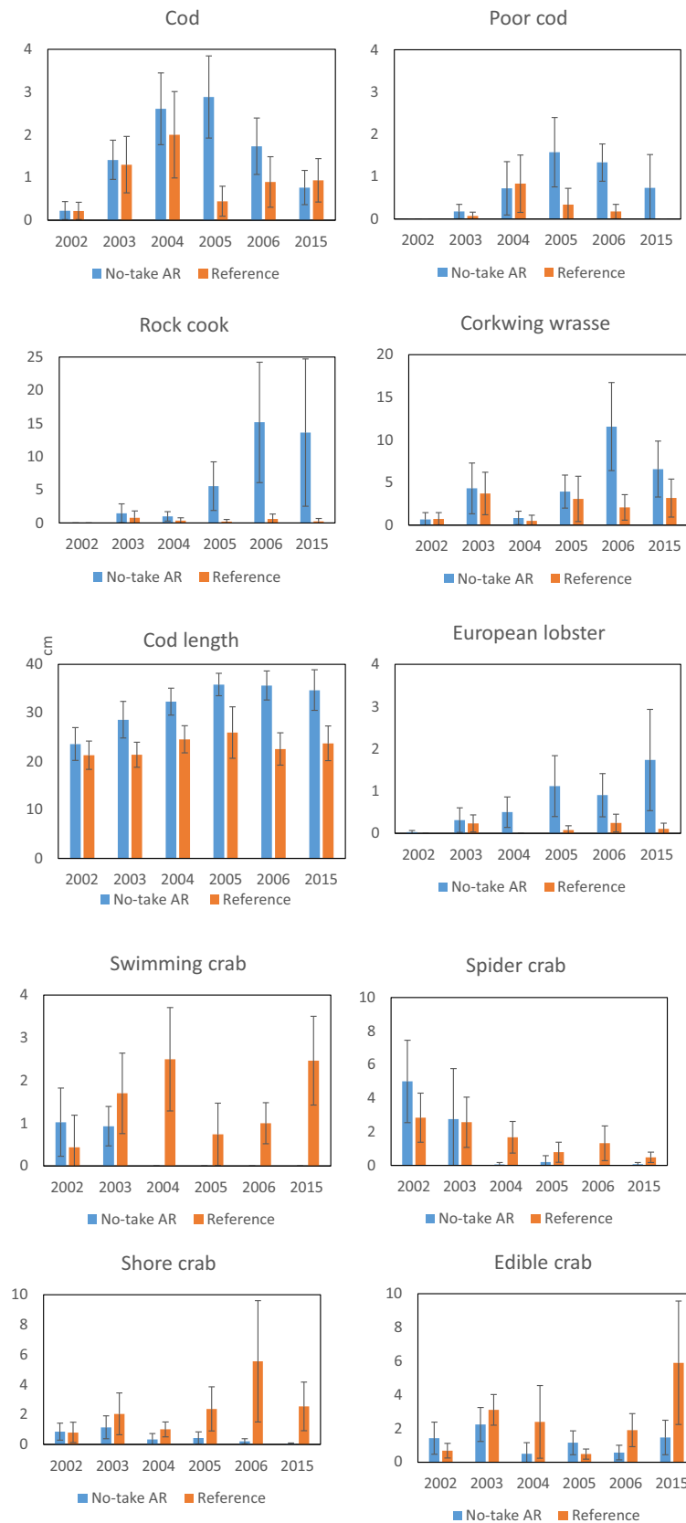
Fig. 4 Fyke net catches (mean abundance per station and night \pm 95% confidence intervals) of predatory fish, mesopredatory fish and decapod crustaceans as well as cod length in the NTAR and in the reference area 2002–2006 + 2015 (all zero values represent no individuals caught)
