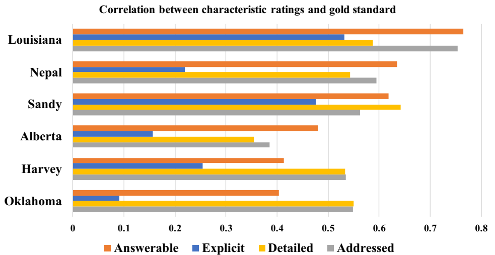
Fig. 2 We observe a positive correlation between the average crowdsourced (non-expert) ratings of the proposed serviceability characteristics and the gold standard annotations of serviceability given by domain experts, according to Pearson Correlation. All correlations are statistically significant at p \leq 0.01 level (2-tailed) except for the case of Explicit Request in the Oklahoma event
