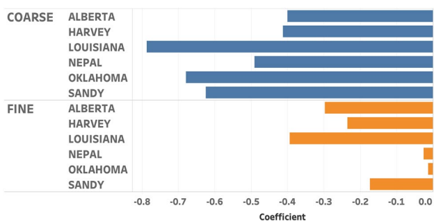
Fig. 5 Pearson correlation coefficients between the cluster rank and cluster size for the resulting clusters of semantic grouping across all events, indicating uniqueness of the higher-ranked requests
