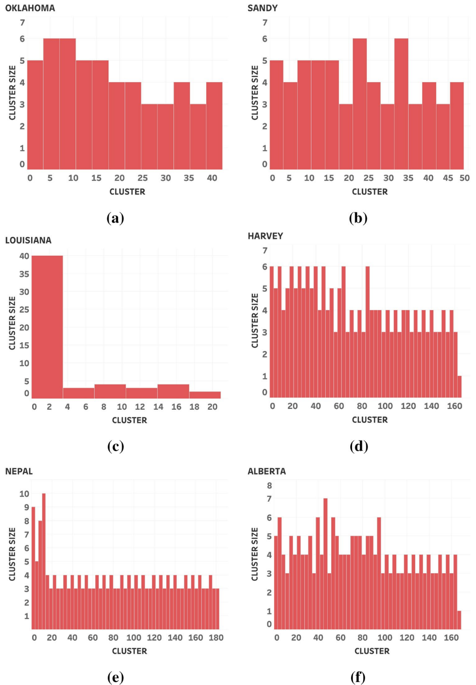
Fig. 3 Histogram of cluster size distribution across events for the results from fine-granularity clustering method
