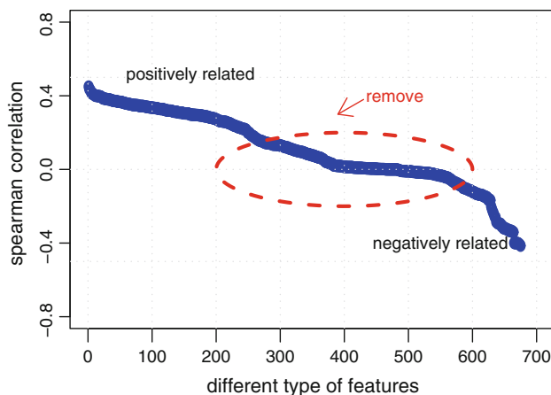
Fig. 2 Positive, negative, and unrelated network features
