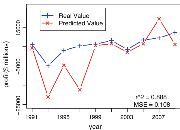
(a) IBM profit prediction.
