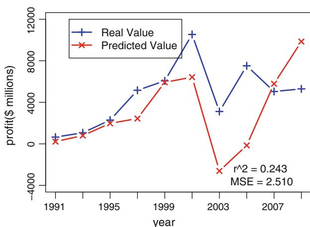
(b) Intel profit prediction.
