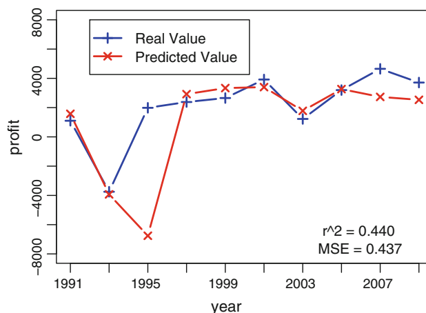
Fig. 4 Prediction of the mean profits of 20 Fortune companies
