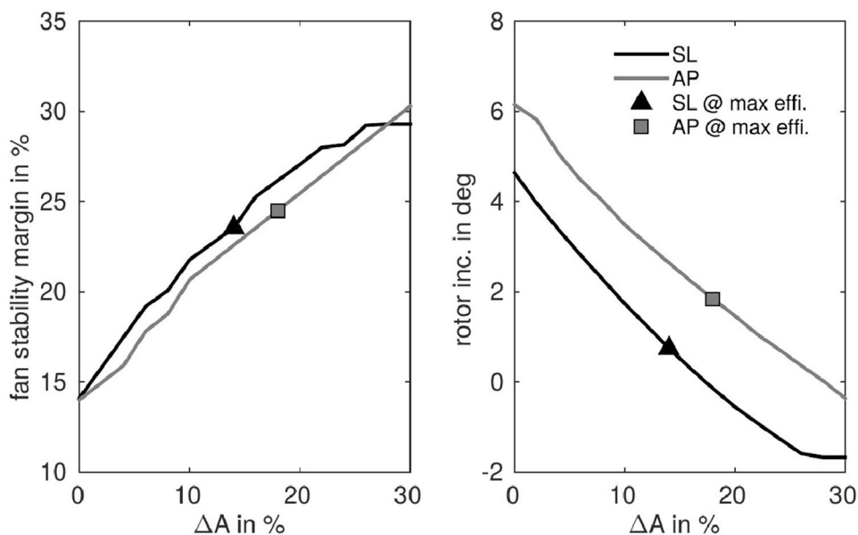
Fig. 12 Variation of fan stability (left) and rotor incidence (right) with nozzle opening
