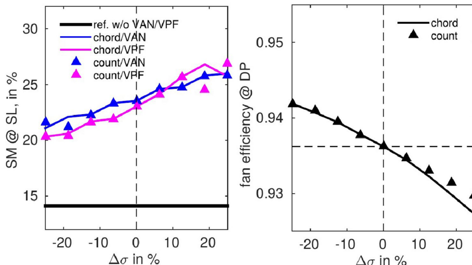
Fig. 22 Impact of a rotor-solidity variation on fan aerodynamic performance: stability margin at SL (left) and isentropic efficiency at DP (right)
