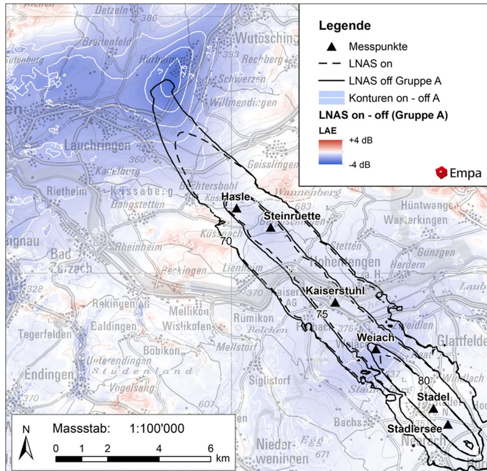
Fig. 11 Footprint differences between LNAS on versus LNAS off based on the weighted sound exposure level L_{AE} footprints for the ATRA flights. Relevant with respect to Swiss noise legislation are the differences within the absolute L_{AE} contours for LNAS on (dashed) and LNAS off (solid). The differences are additionally marked with white contour lines in 0.5 dB steps
