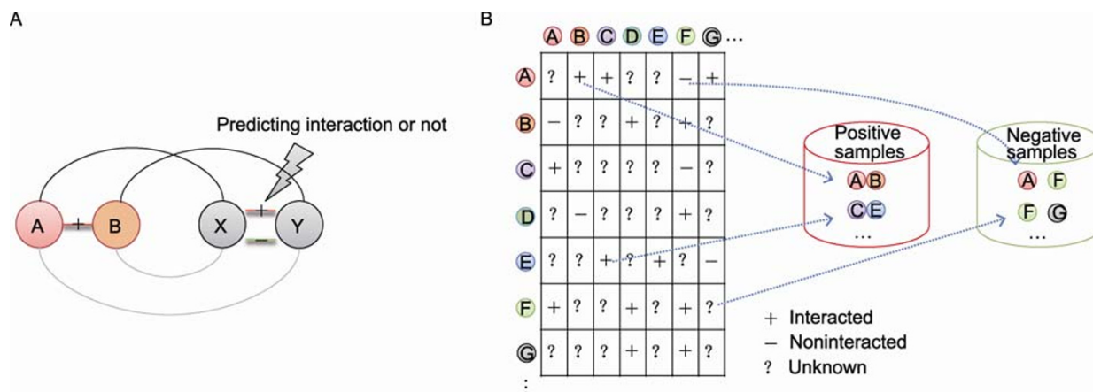
Figure 1. Framework of predicting PPIs. (A) Mapping the interacting proteins to the predicting pairs by directly comparing their similarities (the first group); (B) Constructing positive and negative samples to learn the interaction features for prediction (the second group).
