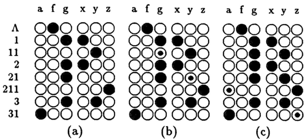
Fig. 3 Computing a unifier by a neural network. Example taken from [13]. The figure depicts the representation of \langle f(x, x, y) = f(g(y), g(g(z)), g(a)) \rangle ; a initially, b after 1 step, and c after 2 steps, where the most recently activated units are half-filled
