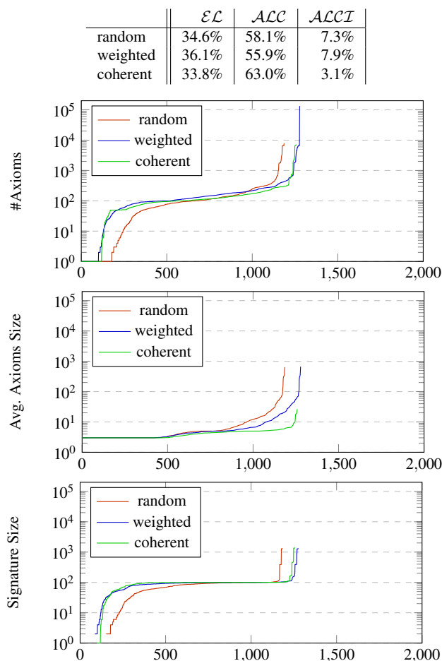
Fig. 4 Uniform interpolants computed by FAME
