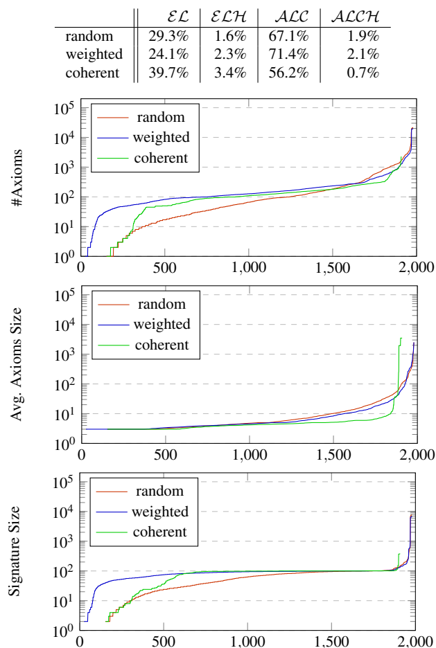
Fig. 5 Uniform interpolants computed by LETHE
