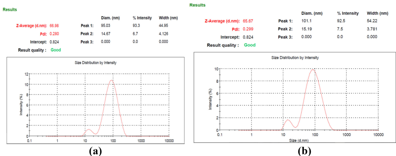
Fig. 6 a DLS result for S3. b DLS result for S1
