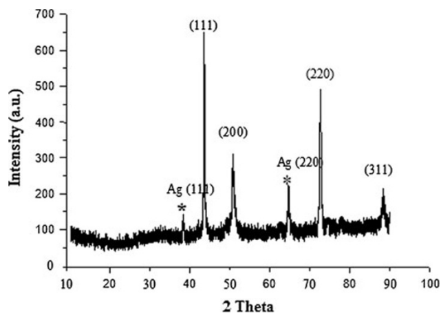
Fig. 4 The XRD pattern of copper nanowires
