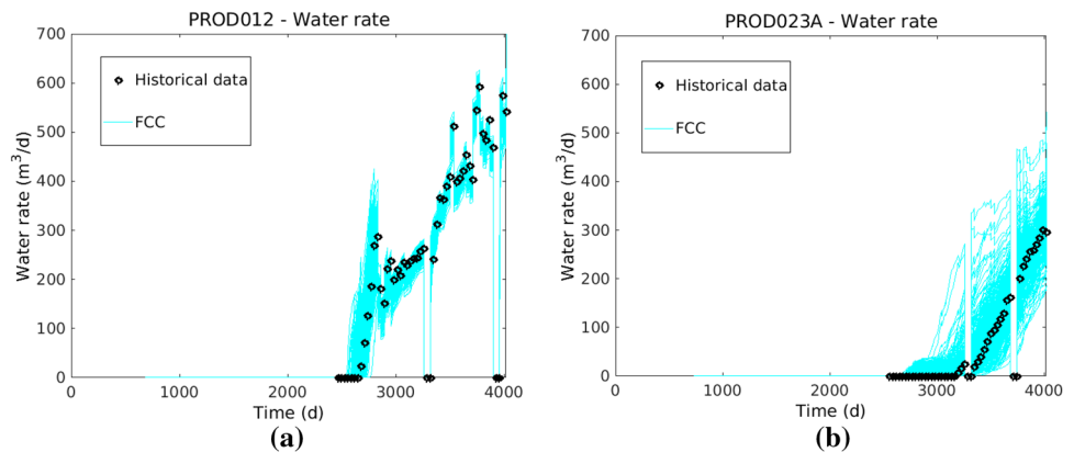
Fig. 4 Water rate: PROD012-FCC (a); and PROD023A-FCC (b)
