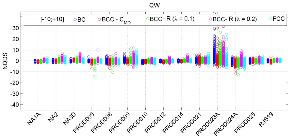
Fig. 3 NQDS for q_w
