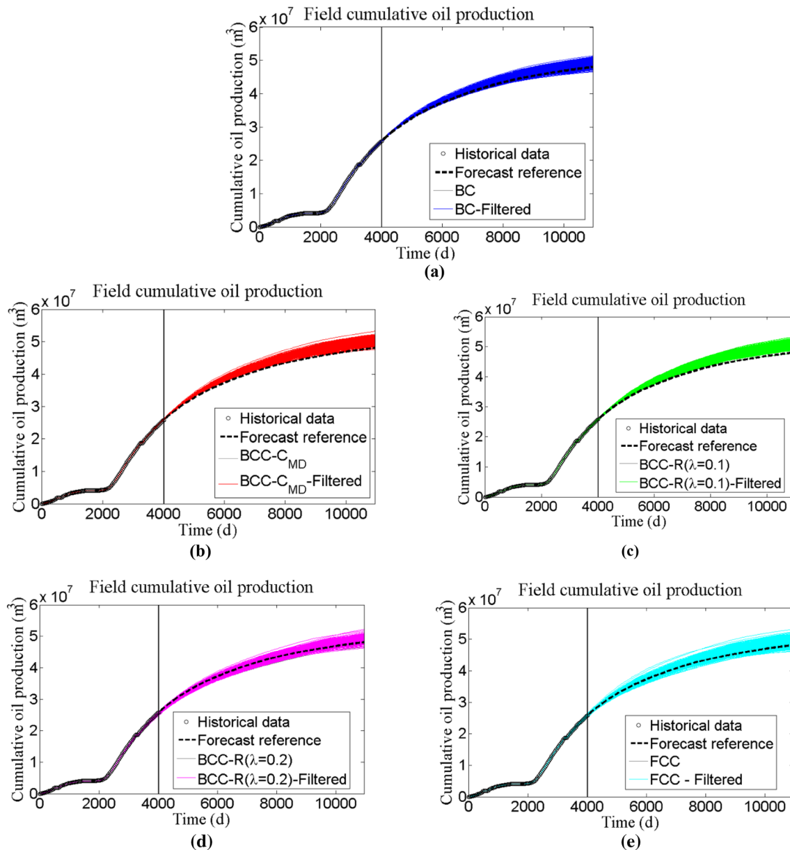
Fig. 8 Field cumulative oil production compared to the forecast reference from the true case: BC (a); BCC- C_{MD} (b); BCC- R ( \lambda=0.1 ) (c); BCC- R ( \lambda=0.2 ) (d); and FCC
