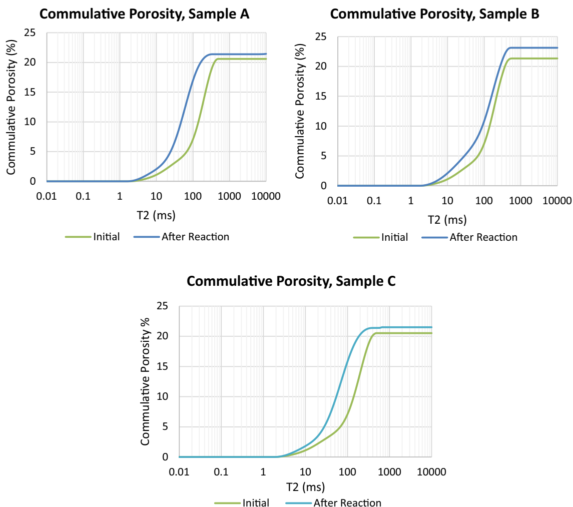
Fig. 15 T2 commulative spectrum of Berea sandstone core samples before and after reaction with chelates
