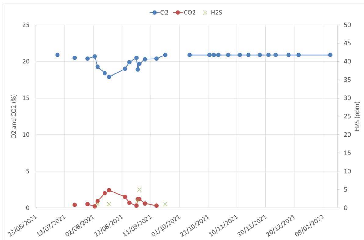
Fig. 7 Process monitoring profile for O 2 , CO 2 , and H 2 S during the composting test
