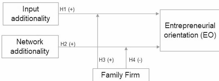
Fig. 1 Research model
