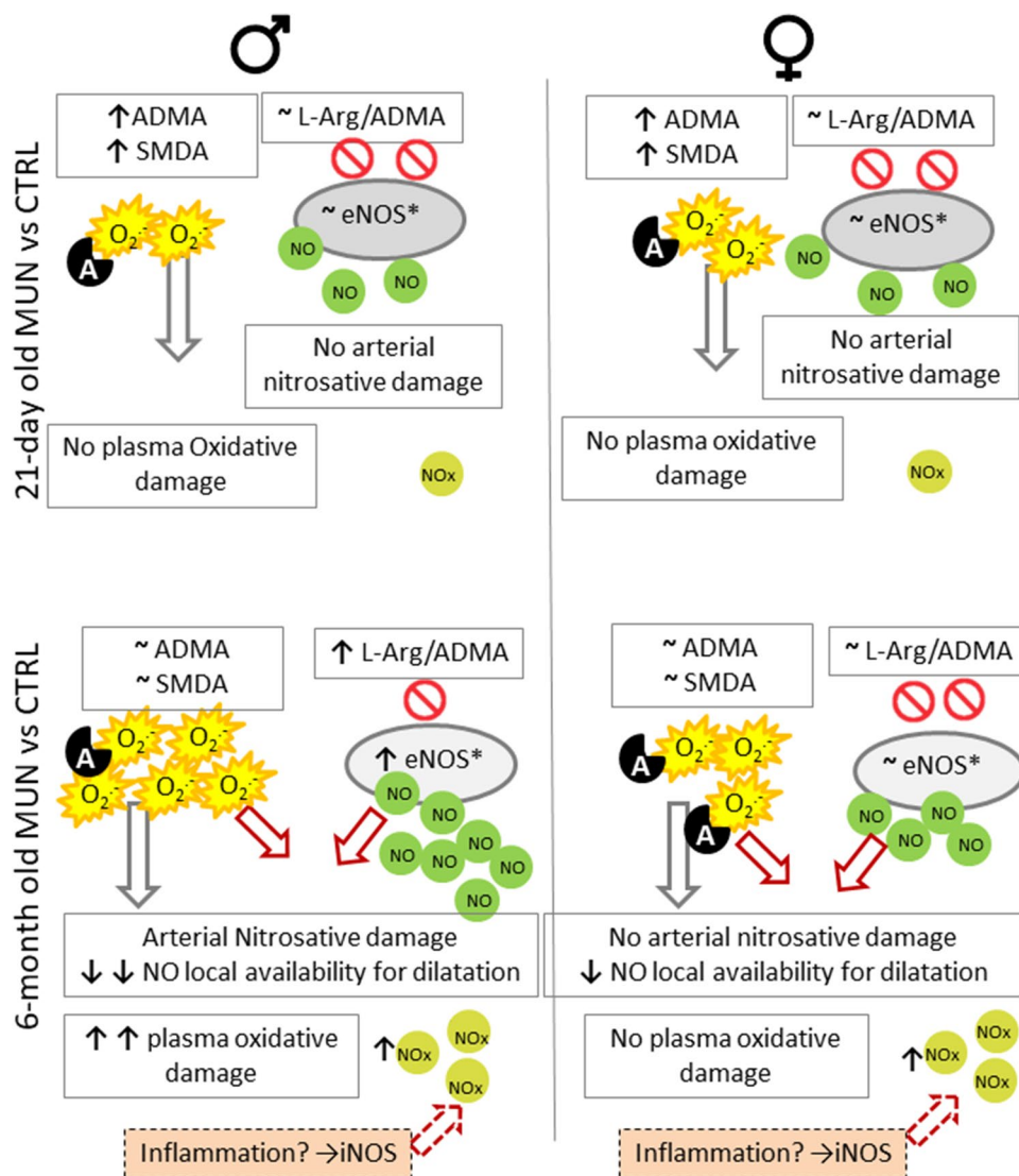
Fig. 7 Schematic diagram depicting the main findings of the study. The figure shows the of alterations related to NO metabolism, oxidative and nitrosative damage from weaning period (21 days) to adult life (6 months) and the comparison between males and females. CTRL, control; NO, nitric oxide; eNOS*, active endothelial Nitric Oxide synthase; NOx, plasma nitrate levels; O 2 - , superoxide anion; A represents antioxidants, likely low in 6-month-old MUN males, as suggested by the lower Nrf2. In the diagram, we also propose iNOS from extravascular cells activated by inflammation as potential source of elevated plasma NOx
