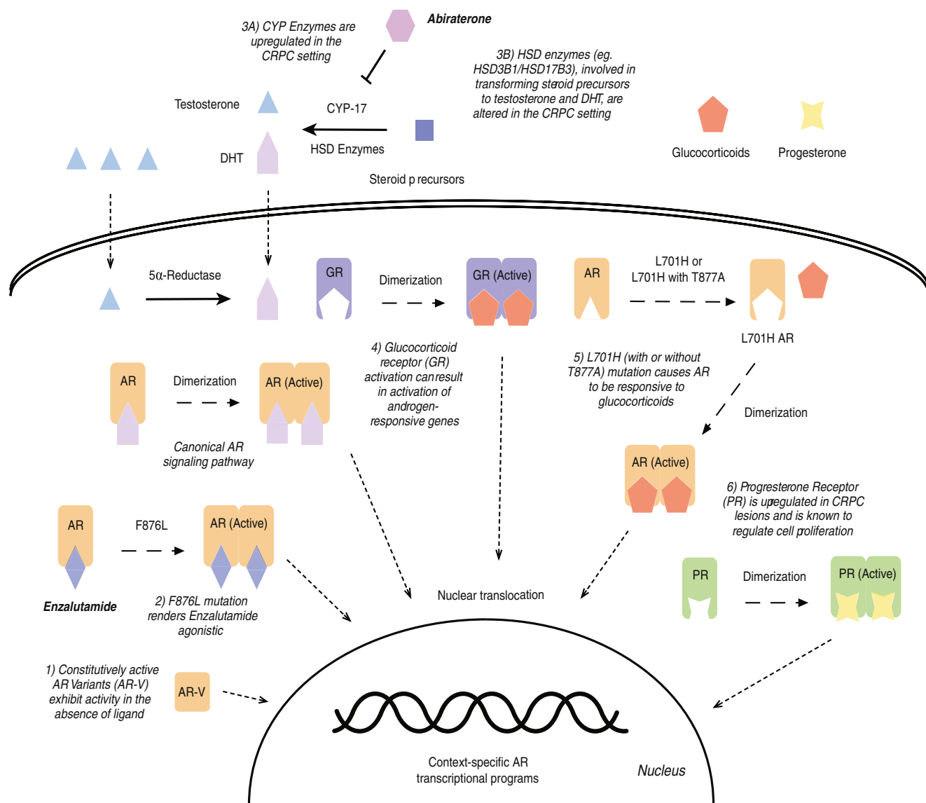
Fig. 2 A summary of candidate molecular alterations leading to the return of AR signaling in spite of treatment with enzalutamide and abiraterone. These alterations include 1 androgen receptor splice variants, 2 AR F876L mutation, 3 steroidogenic enzymes, 4 glucocorticoid receptor overexpression, 5 AR L701H mutation, and 6 progesterone receptor
