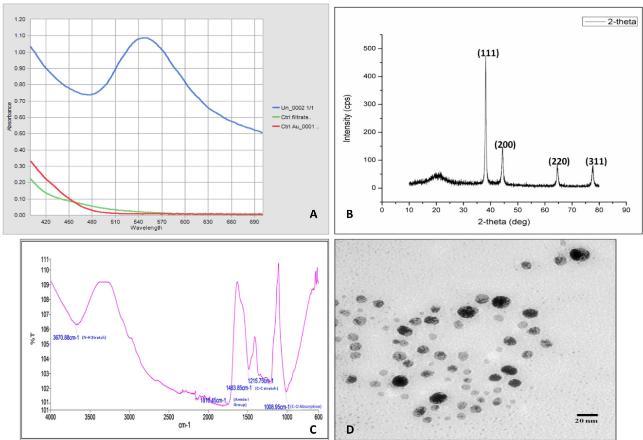
Fig. 4 Graphs depicting characterization methods of gold nanoparticles (AuNPs)
