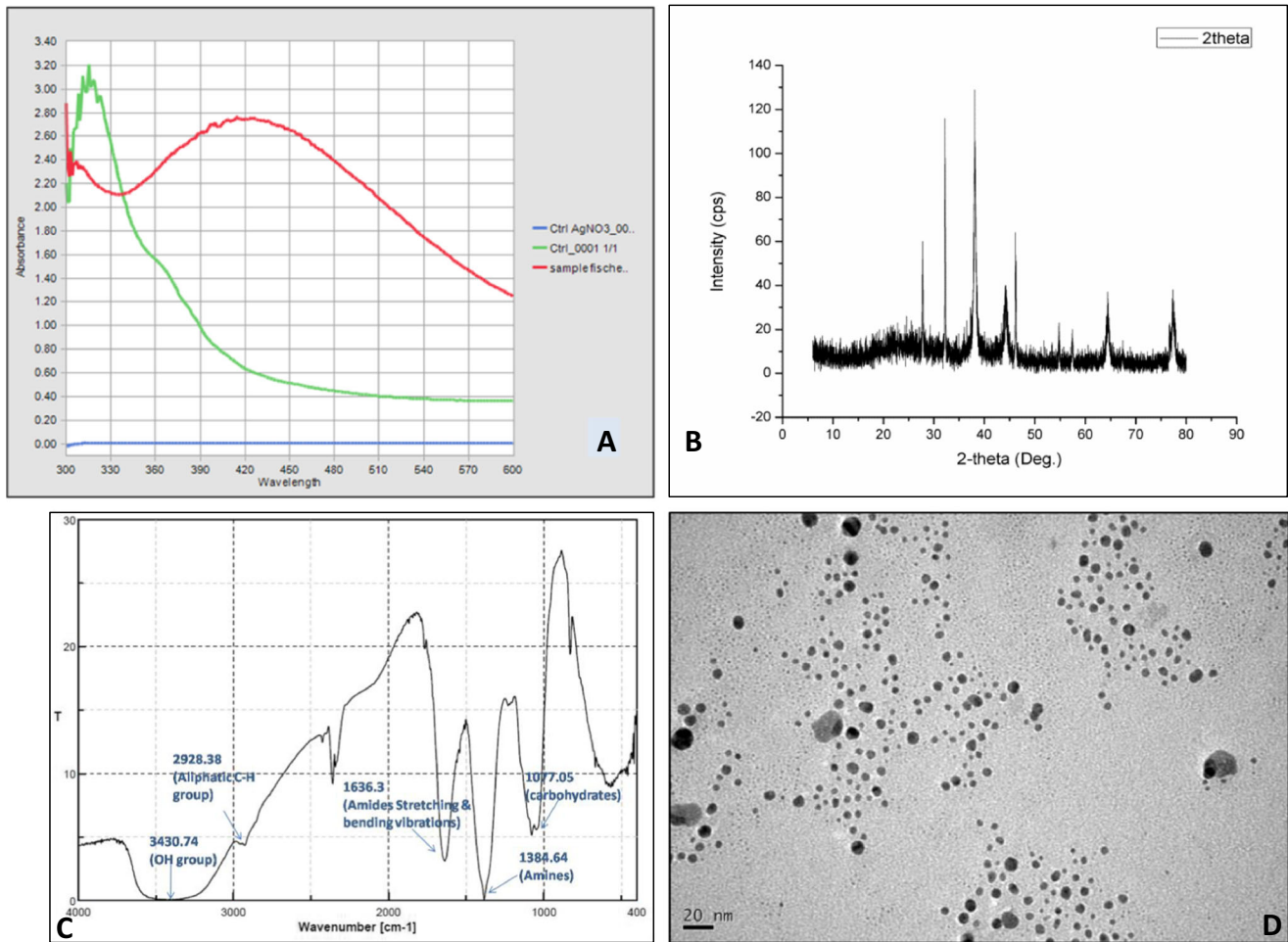
Fig. 3 Illustration of various characterization methods of silver nanoparticles (AgNPs)
