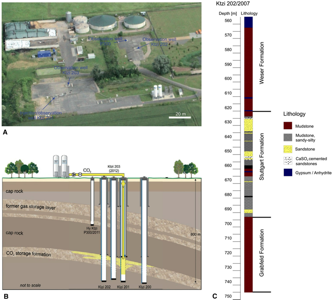
Fig. 1 a Aerial view with scientific infrastructure at the Ketzin CO 2 injection site in June 2013 (changed after Martens et al. 2014). b Schematic cross section through the Ketzin CO 2 storage site showing the injection well and the two monitoring wells (courtesy to
