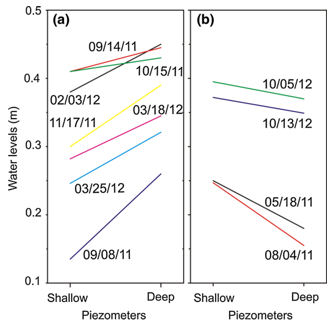
Fig. 8 Water levels in piezometers PZS (shallow) and PZD (deep) indicating the direction of groundwater flow in canal bed at select times during the monitoring periods. a Upward groundwater flow direction, b downward groundwater flow direction
