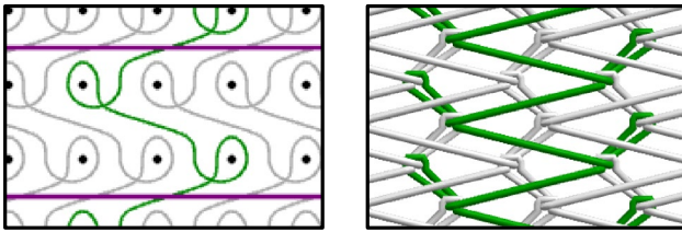
Fig. 15 Cord lap. Pattern draft (left) and CAD image (right)
