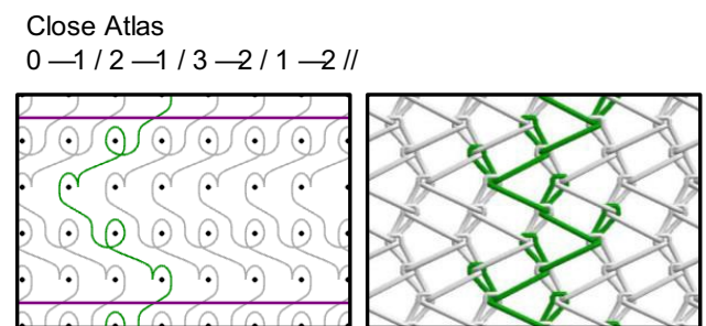
Fig. 13 Atlas lap. Pattern draft (left) and CAD image (right)
