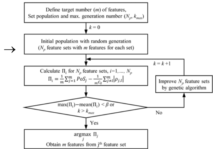
Fig. 9 Feature selection procedure using the GA
