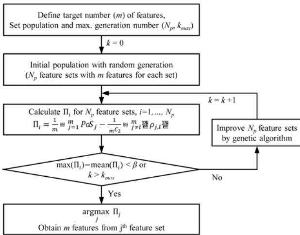
Fig. 9 Feature selection procedure using the GA
