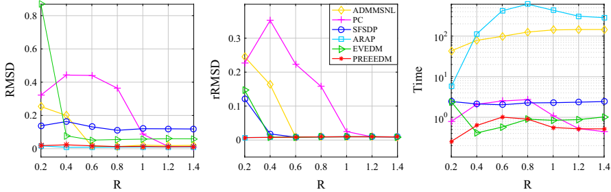
Fig. 3 Average results for Example 1 with n = 200, m = 4, nf = 0.1
