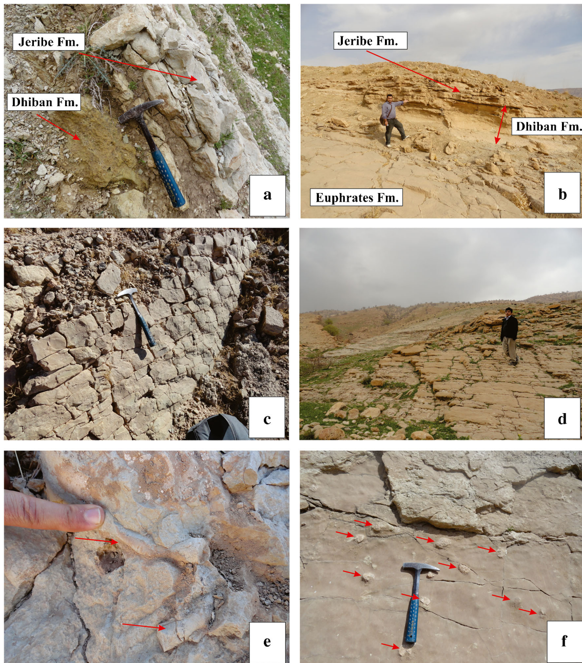
Fig. 6 Representative outcrop photographs of the Dhiban and Jeribe Formations. a Yellowish evaporitic carbonate of the Dhiban Formation between the Euphrates and Jeribe Formations in the Takiya section, which is only 10 cm thick and overlain by the carbonate of the Jeribe Formation. b Evaporitic carbonate of the Dhiban Formation between the Euphrates
