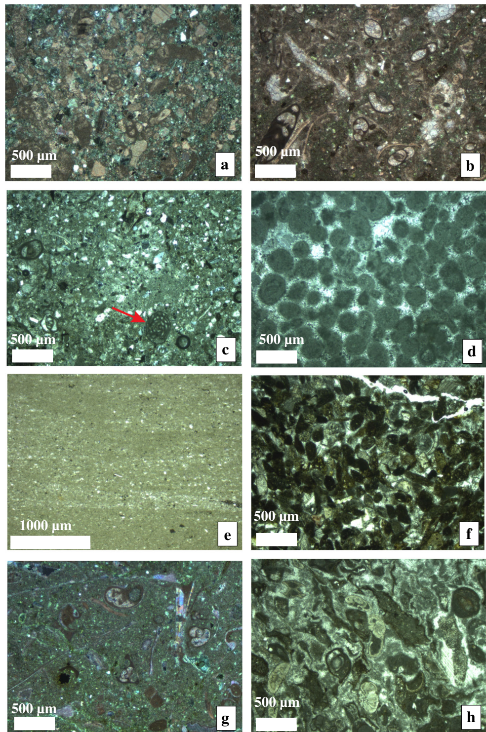
Fig. 7 Representative photomicrographs of the Euphrates and Jeribe Formations. a Reworked-bioclasic grainstone microfacies E1, which belongs to the brecciated carbonate unit of the Euphrates Formation in the Darbandikhan section, showing reworked fossils in an arenitic ground mass. b Bioclasic miliolid packstone microfacies E2 of the Euphrates Formation, Basara section. c Bioclasic miliolid packstone to grainstone microfacies E2 of the Euphrates Formation in the Basara section, showing the Early (Lower) Miocene index fossil, Borelis melo melo . d Ooidal grainstone microfacies E4 of the top of the Euphrates Formation, Basara section. e Calcareous mudstone microfacies J1 of the yellowish-marl of the Jeribe Formation in the Takiya section. f Bioclasic-peloidal grainstone microfacies J2 of the Jeribe Formation. g Miliolid packstone microfacies J3 of the Jeribe Formation, Mamlaha section. h Miliolid-rotaliids packstone microfacies J4 of the Jeribe Formation in the Basara section
