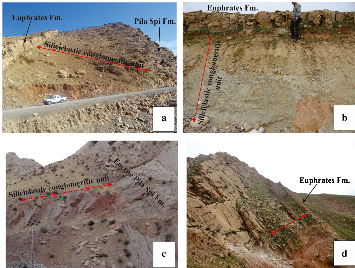
Fig. 4 Representative outcrop photographs of the siliciclastic conglomeritic unit. a Basara section. b Hazar Kani section. c Darbandikhan section. d Takiya section. This unit is overlain by the carbonate of the Euphrates Formation
