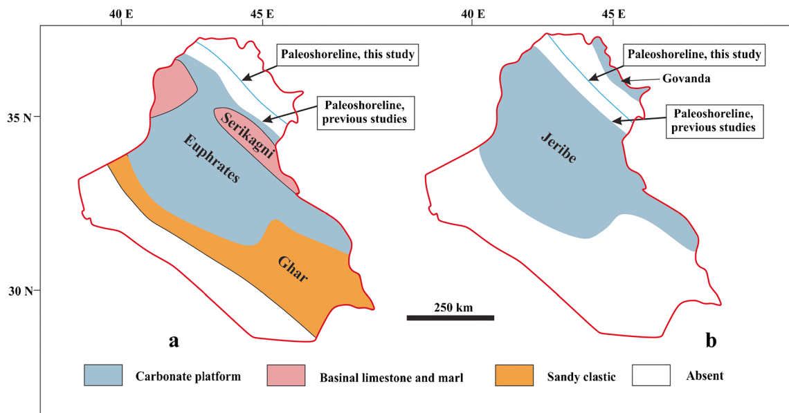
Fig. 9 Palaeogeography of Iraq. a During latest Chattian to early Aquitanian, showing the deposition of the Euphrates and Serikagni Formations after Aqrawi et al. (2010), and the new palaeoshoreline in
