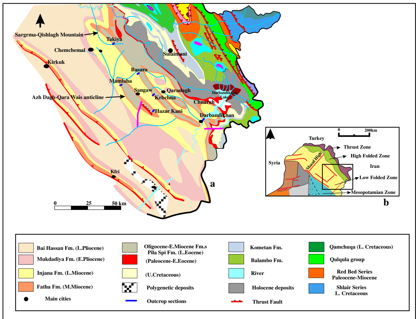
Fig. 1 Geological maps of the study area. a Geological map illustrating the study area and the studied sections. b Structural map of northern Iraq including Kurdistan structural elements and the study area (Aqrawi et al. 2010)
