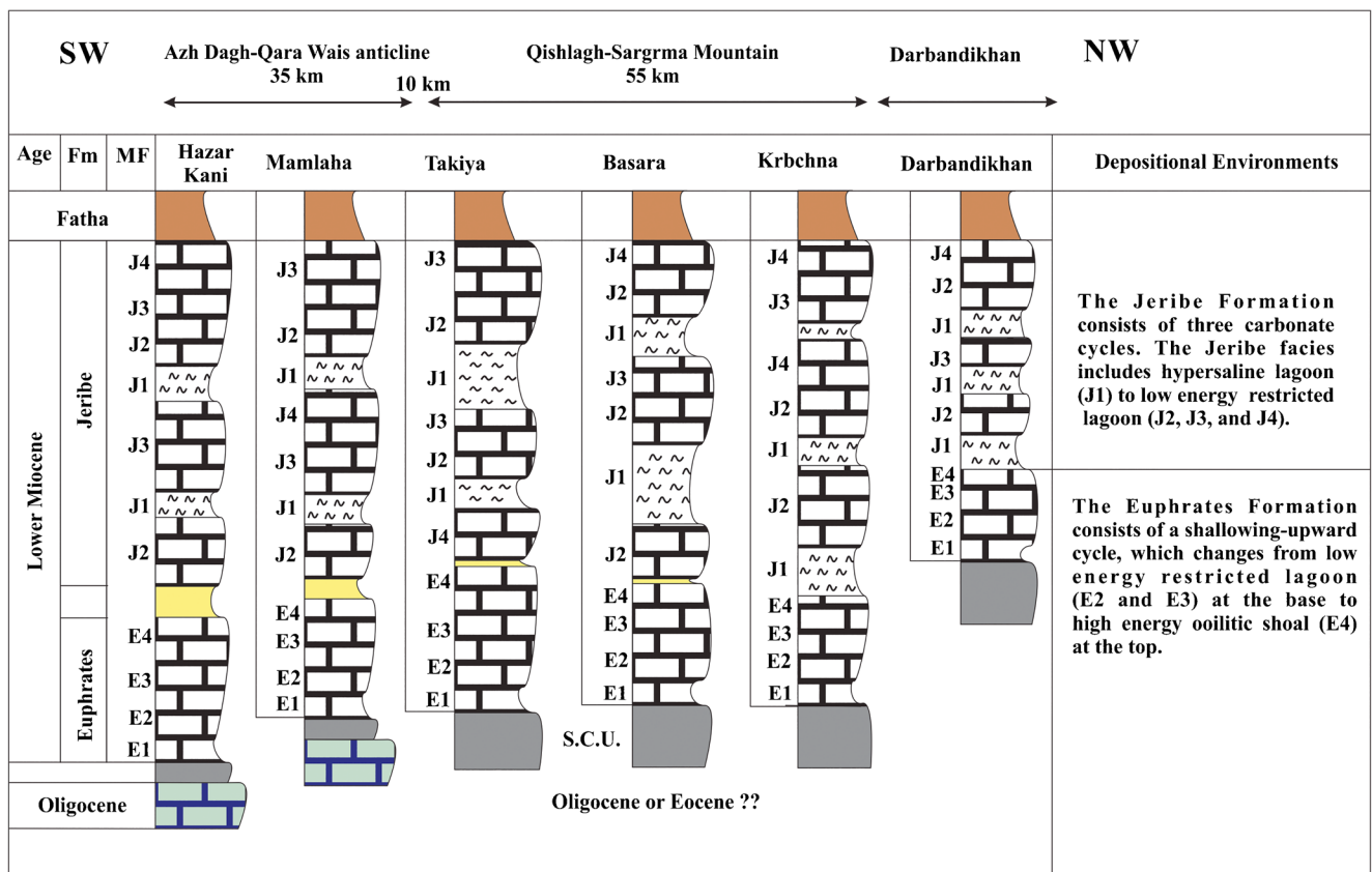
Fig. 10 Lithostratigraphic correlations of the Lower (Early) Miocene formations in the studied areas, Qishlagh-Sargrma, Darbandikhan, and Azh Dagh-Qara Wais, illustrating the facies distributions and depositional
