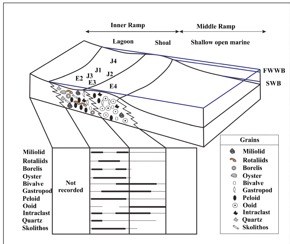
Fig. 8 Schematic diagram of the depositional ramp model of the Early (Lower) Miocene formations in the Kurdistan Region. FWWB, fair weather wave base; SWB, storm wave base
