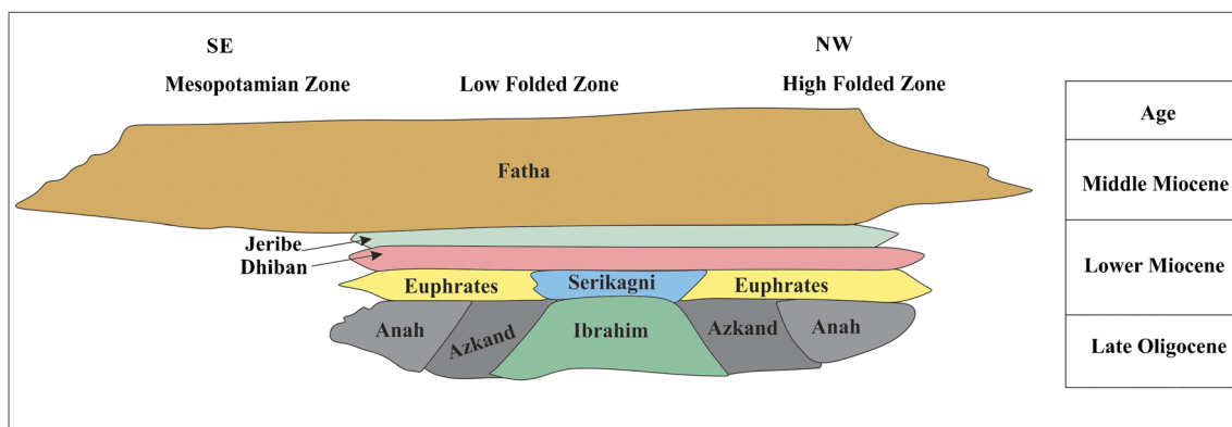
Fig. 2 Chronostratigraphic chart of Iraq (after van Bellen et al. (1959) and modified by Aqrawi et al. (2010))
