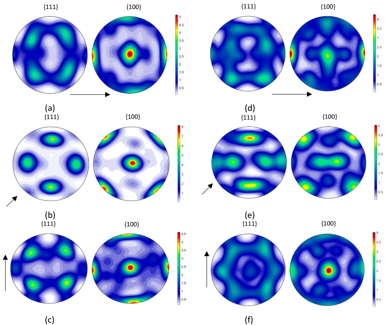
Fig. 14 {111} and {100} pole figures obtained from the EBSD measurements performed on samples taken at the middle (left column) and at the top of fully draw cup (right column) respectively along (see
