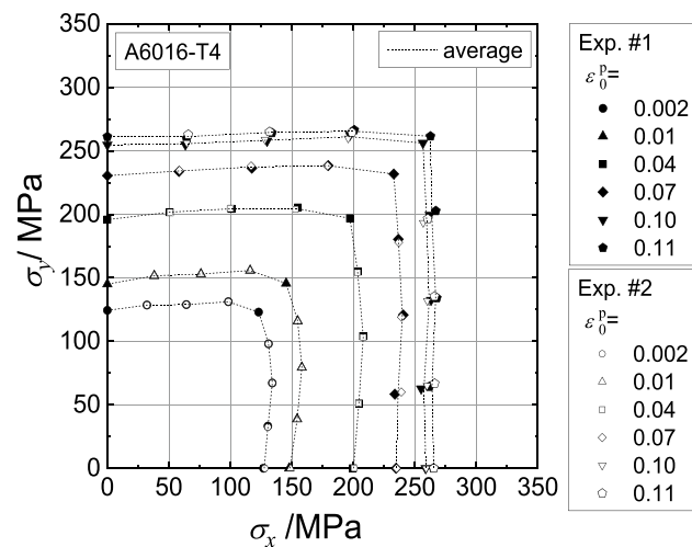
Fig. 8 Stress points forming contours of plastic work at different levels of \epsilon_0^p
