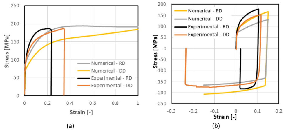
Fig. 43 VPSC simulations compared with the: a monotonic and b reversed shear tests of ULiège, used for the validation of the model
