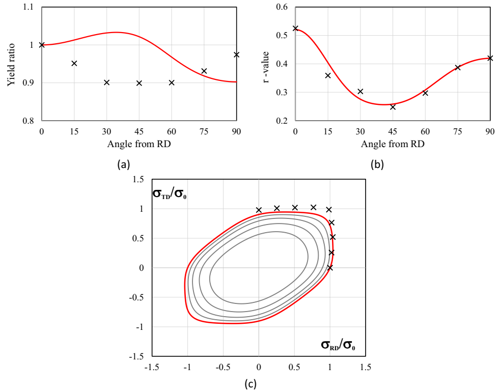
Fig. 56 Predicted results by CB2001 criterion (Eq. 15): a Tensile flow stresses; b Lankford coefficients; c Yield surface section in the biaxial plane ( \sigma_{RD}, \sigma_{TD} ) (with \sigma_{xy}/\sigma_0 = 0, 0.2, 0.3, 0.4, 0.5 ). Data represented by symbols. All stresses are normalized by the yield stress along the rolling direction, \sigma_0
