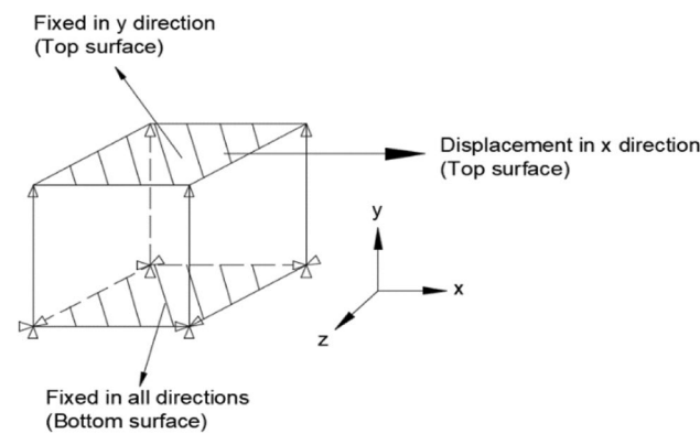
Fig. 69 Reversal shear boundary conditions on a representative single element
