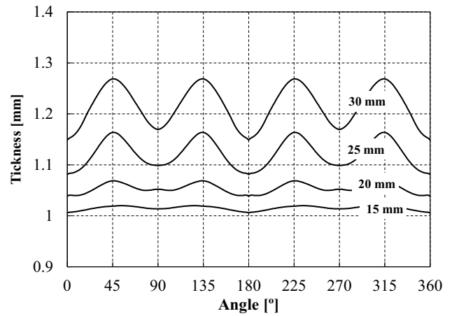
Fig. 114 Evolution of the thickness along the cup circumference at different heights H=15, 20, 25 and 30 mm, respectively from the cup bottom, by Caz2018polycrys model based on the Caz2018singlecrys model (Eqs. 30–32)
