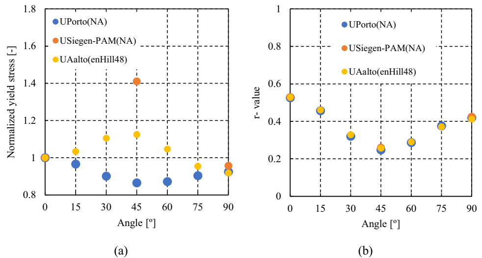
Fig. 79 Predicted FE results by (non-associated flow rule) Hill48 criterion with constant or evolving anisotropy parameters identified in “Hill48 and non-associated flow rule” Section (Eqs. 71): a uniaxial tensile flow stresses, b Lankford coefficients ( r -values). Note that for UAalto (enHill48) the results are plotted only for an equivalent plastic strain of 0.18
