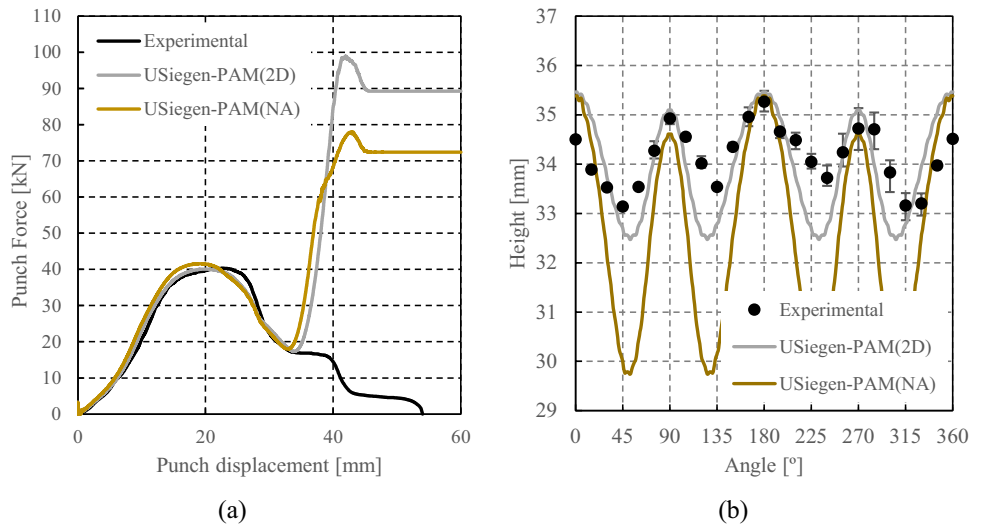
Fig. 80 Comparison between experimental and predicted results with shell elements and Hill48 criterion with associated flow rule (data set Table 22-line 1) and non-associated flow rule (data set computed by Eqs. (71) for constant anisotropy properties (see Tables 4 and 5): a punch force-displacement, b earing profile
