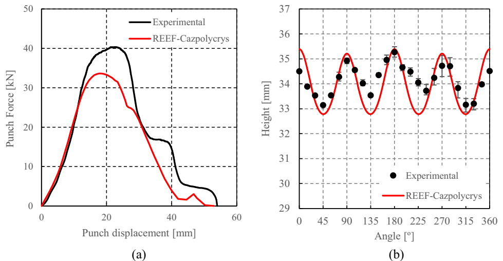
Fig. 113 Comparison between experimental and predicted results by Caz2018polycrys model based on Caz2018singlecrys (Eqs. 30–32): a punch force-displacement, b earing profile
