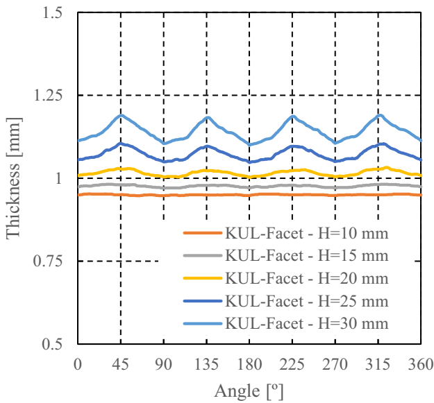
Fig. 112 Evolution of the thickness along the cup circumference at different heights H=15, 20, 25 and 30 mm from the cup bottom, by the Facet-3D model identified by ALAMEL (see “Facet-3D model” Section)
