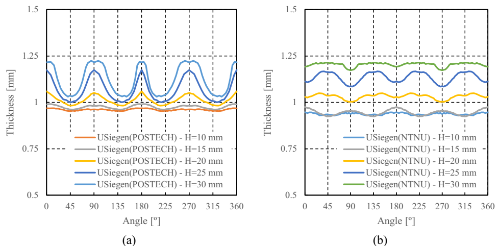
Fig. 86 Evolution of the thickness along the cup circumference at different heights H = 15, 20, 25 and 30 mm from the cup bottom, using LS-DYNA (built-in; USiegen) and the set of anisotropy coefficients provided by: a POSTECH and b NTNU (see “Yld2000-2D and Yld 2004-18p” Section (Table 28))
