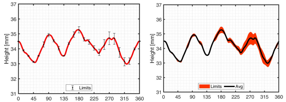
Fig. 21 Evolution of average cup height for different angles
