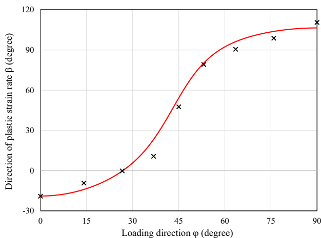
Fig. 57 Predicted direction of the plastic strain-rate \beta = \arctan(D_{yy}^p/D_{xx}^p) for biaxial loading at \phi = \arctan(\sigma_{RD}/\sigma_{TD}) by CB2001 criterion. Data represented by cross symbols
