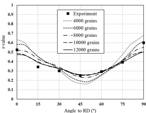
Fig. 30 Effect of number of grains in the discrete texture on the r -values obtained by ALAMEL. This texture is generated by making the measured EBSD texture continuous with \varphi_0 = 3^\circ and L_{\max} = 22 followed by a statistical discretization procedure described in [94]
