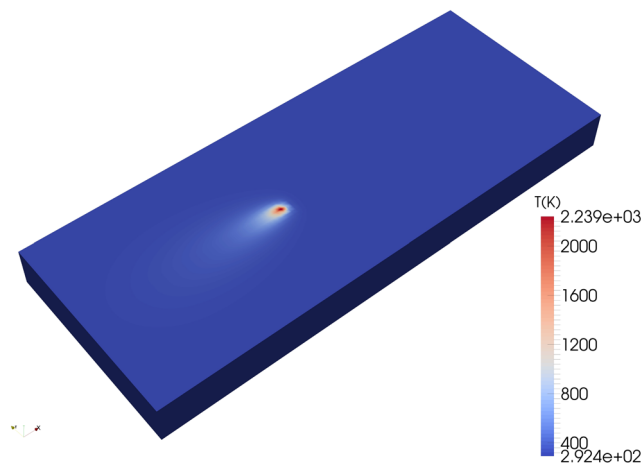
Fig. 3 Temperature field at a given time t , with the source moving from the left boundary towards the right one
