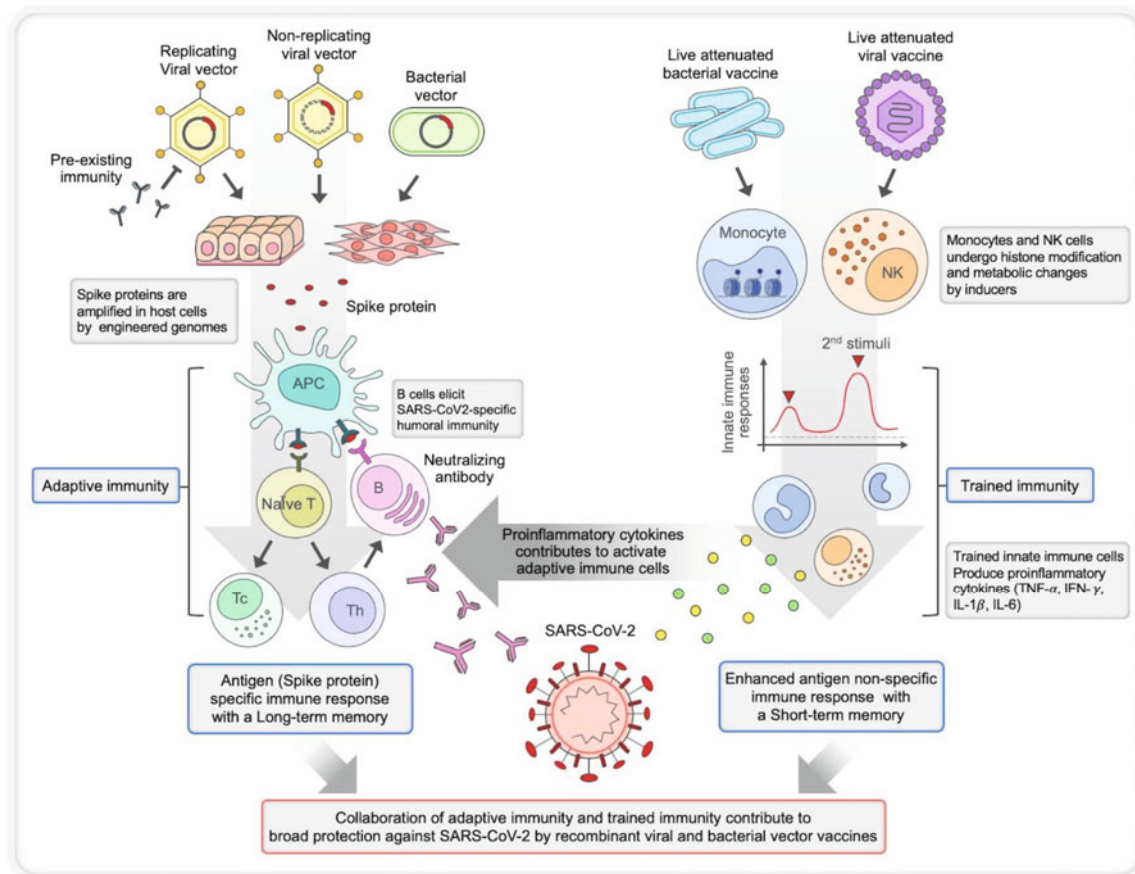
Fig. 1. COVID-19 vaccines based on recombinant viral and bacterial delivery systems can provide a better protection via combinatorial effect of adaptive and trained immunity. First, they possess various pattern-associated molecular patterns (PAMPs) leading to adjuvant free vaccination. Second, they can induce adaptive T cell-mediated and humoral immune responses specific to SARS-CoV-2 infection. Third, they can induce broad-spectrum off-target vaccine effects via trained immunity, providing a better protective effect even against vaccine escape variants.
