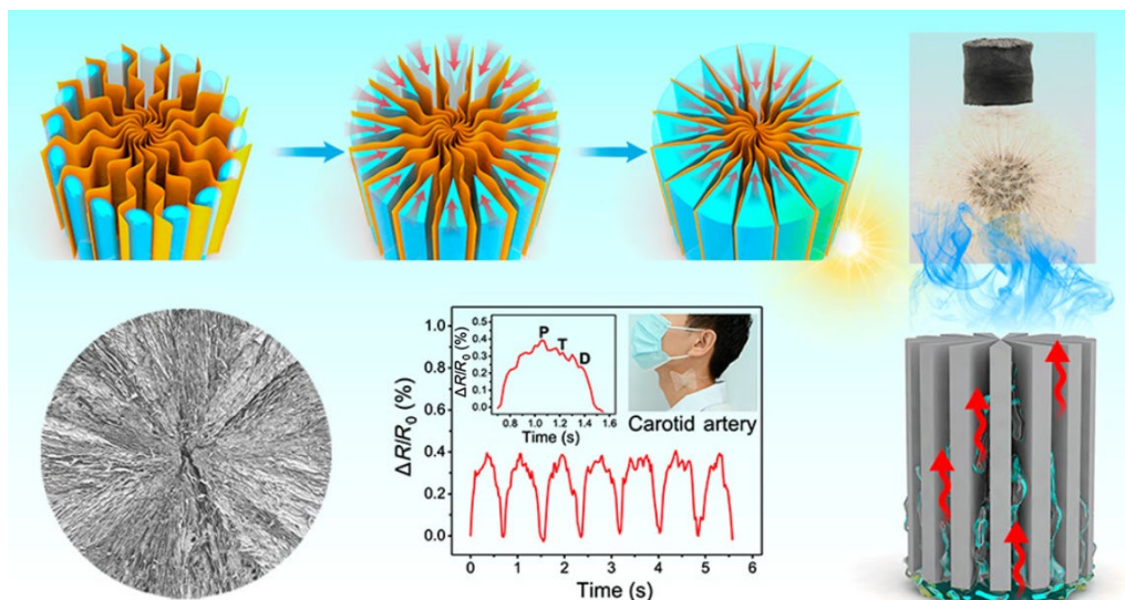
Figure 16 The MXene/polyimide aerogels-based piezoresistive sensor for human motion monitoring. The fabrication of xylem-like architecture (top). SEM image (bottom left). The sensing performance for monitoring the carotid artery (bottom middle). Demonstration of such structure for water steam collection (bottom right). Reproduced with permission from Ref. [225], © American Chemical Society 2022.
