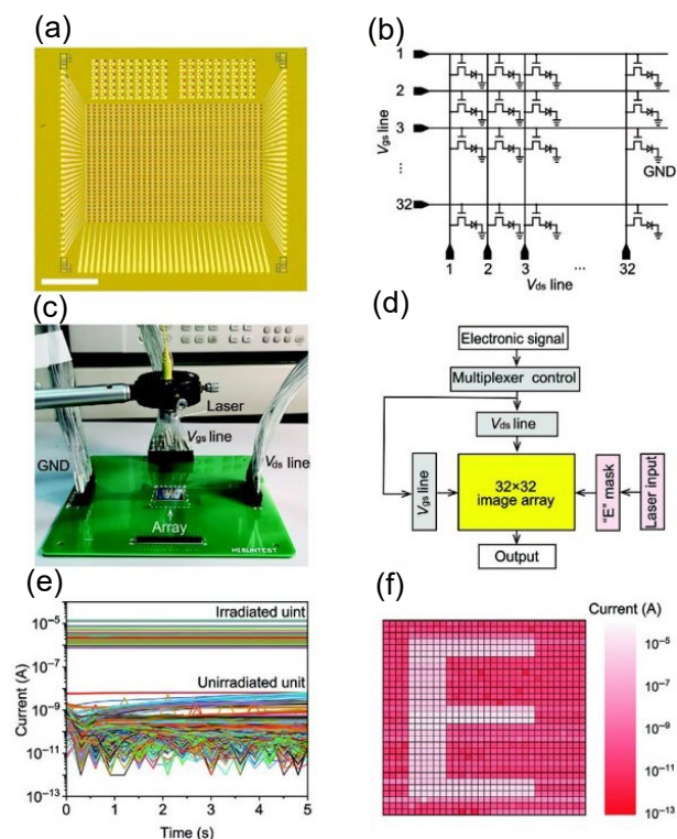
Figure 4 MXene/Si heterostructure-based image sensor. (a) Photograph of an image sensor of 32 \times 32 pixel photodetectors. (b) Circuit diagram, (c) photograph, and (d) workflow diagram of the image sensor by a multiplexer technology. (c) Test the array chip using the laser and a shade cover on top of the array. The V_{\text{gs}} , V_{\text{ds}} , and ground wires (GND, i.e., the chip substrate) are connected to the measuring system. (d) The electrical signal input is controlled by the multiplexer and then generated by the V_{\text{ds}} line to generate an array of 1,024 pixels. (e) The 1,024 pieces of drain current curves from each pixel photodetector. The higher current ( 10^{-6} A) occurs at the irradiated photodetector while the lower current ( 10^{-9} A) emerges at the dark condition with the light selectively illumination inside the capital E projection. (f) The image detection of E capital alphabet by the 1,024 pixels of drain current after a current mapping. Reproduced with permission from Ref. [140], © Wiley-VCH GmbH 2022.
