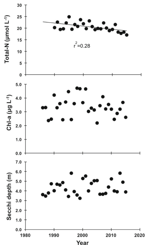
Fig. 2 Regional monitoring data. Changes in seasonal averages (April–September) of organic and inorganic nitrogen concentration (total-N), chlorophyll- a concentration (Chl- a ), and Secchi depth at the monitoring station Instö Ränna 1986–2015. The trend line denotes a significant decrease of total-N over the study period (Table 2)
