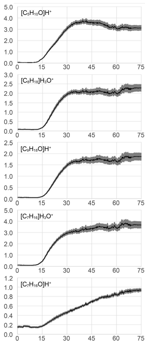
Fig. 4 The changes of concentration (ppm v , horizontal axis) of selected ions during the incubation of rapeseed oil at 180 °C over a period of 75 min (horizontal axis) measured in real time using PTR-TOFMS. The selected ions correspond to protonated compounds: 2-pentanone, octane, nonanal, heptane and 1-heptanol, respectively
