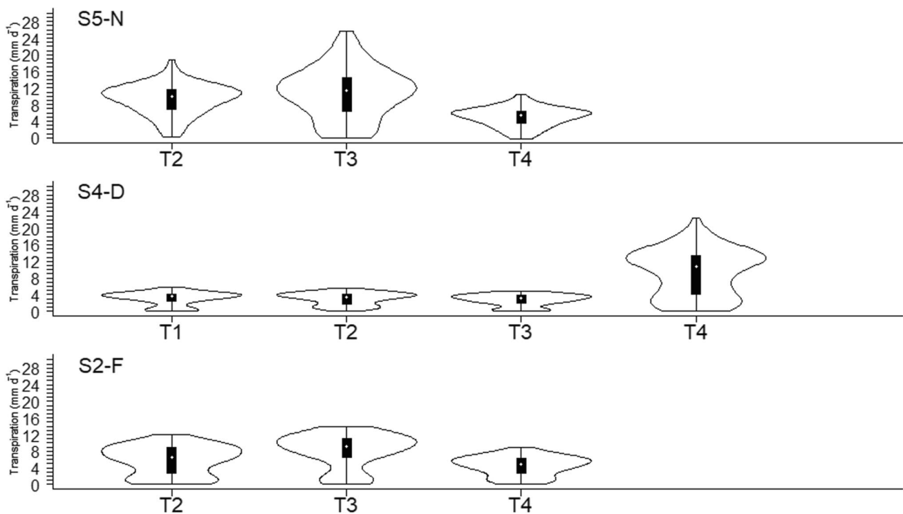
Fig. 3 Distribution plot of daily mean transpiration (in \text{mm d}^{-1} ) of monitored trees grouped per site. On the site with higher groundwater level (S5-N), the selected trees were: S5-T2 (DBH class=II), S5-T4, (DBH class=I), and tree S5-T3 (DBH class=III). On the site with low groundwater table (S4-D), the selected trees were S4-T1
