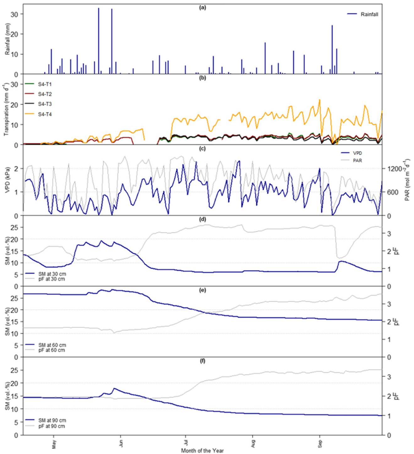
Fig. 5 Daily mean transpiration in relation to meteorological and soil-related conditions for the site with low groundwater level (S4-D). a Cumulative daily rainfall (mm). b Daily course of transpiration (mm d -1 ) for all the analyzed trees within the site. c Daily vapor pressure deficit (VPD, in kPa) and diurnal cumulative photosynthetic active
