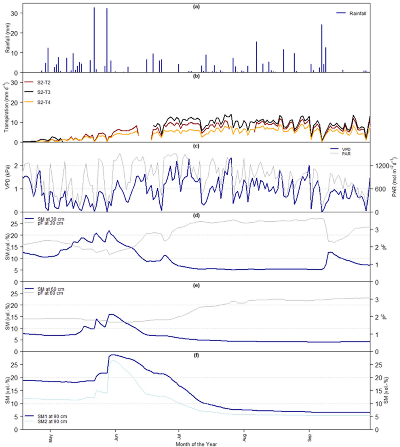
Fig. 6 Daily mean transpiration in relation to meteorological and soil-related conditions for the site with fluctuating groundwater level (S2-F). a Cumulative daily rainfall (mm). b Daily mean transpiration ( \text{mm d}^{-1} ) for all the analyzed trees within the site. c Vapor pressure deficit (VPD, in kPa) and diurnal cumulative photosynthetic active radia-
