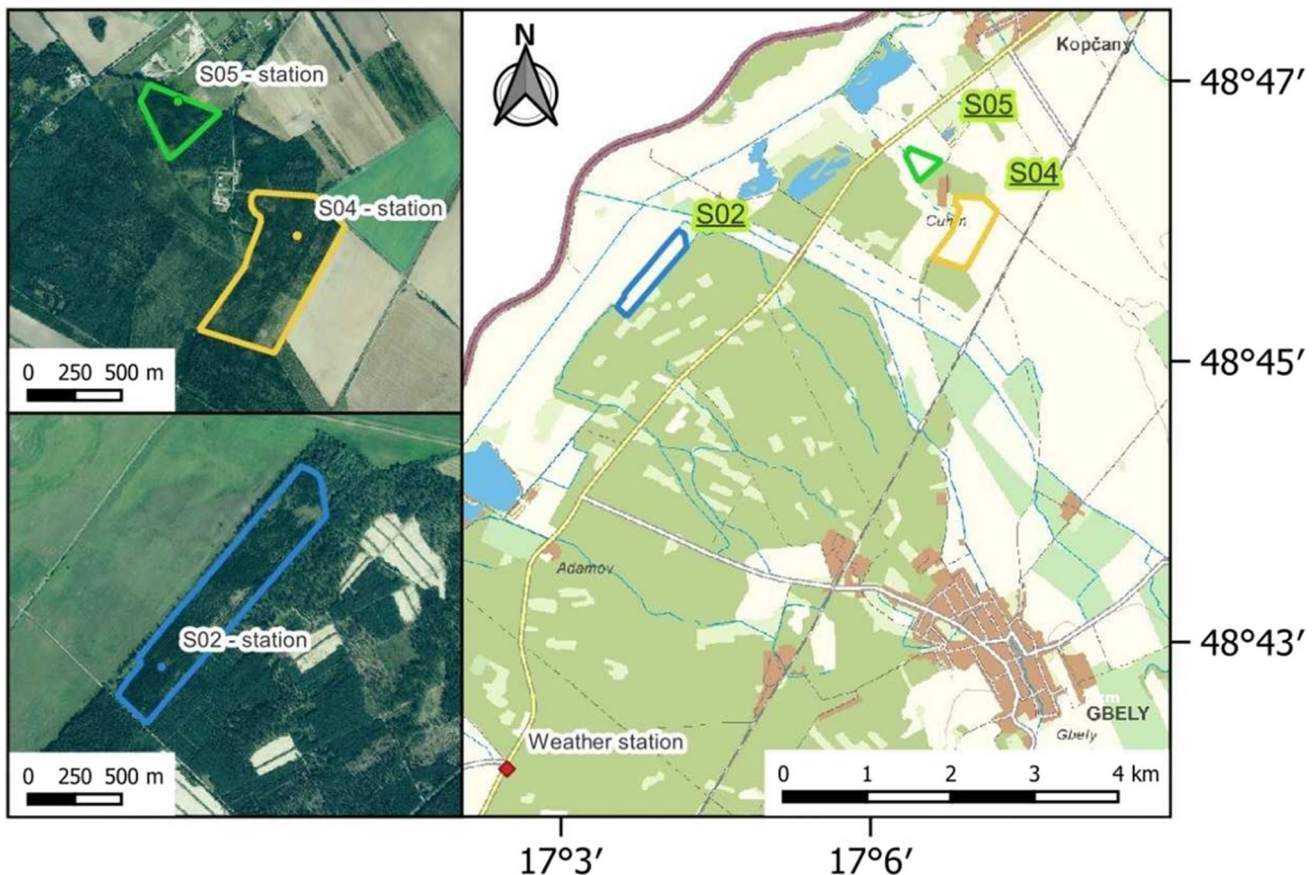
Fig. 1 Location of study area and experimental plots near the village of Kopčany, Skalica region, western Slovakia
