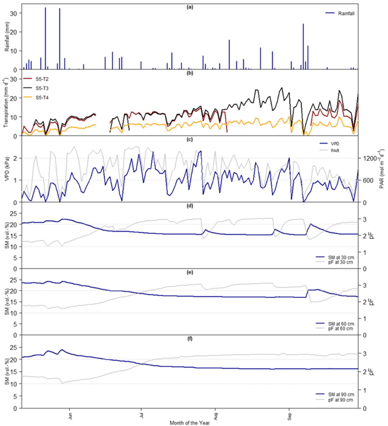
Fig. 4 Daily mean transpiration in relation to meteorological and soil-related conditions for the site with higher groundwater level (S5-N). a Cumulative daily rainfall (mm). b Daily course of transpiration (mm d -1 ) for all the analyzed trees. c Daily vapor pressure deficit (VPD, in kPa) and diurnal cumulative photosynthetic active radiation (PAR, in
