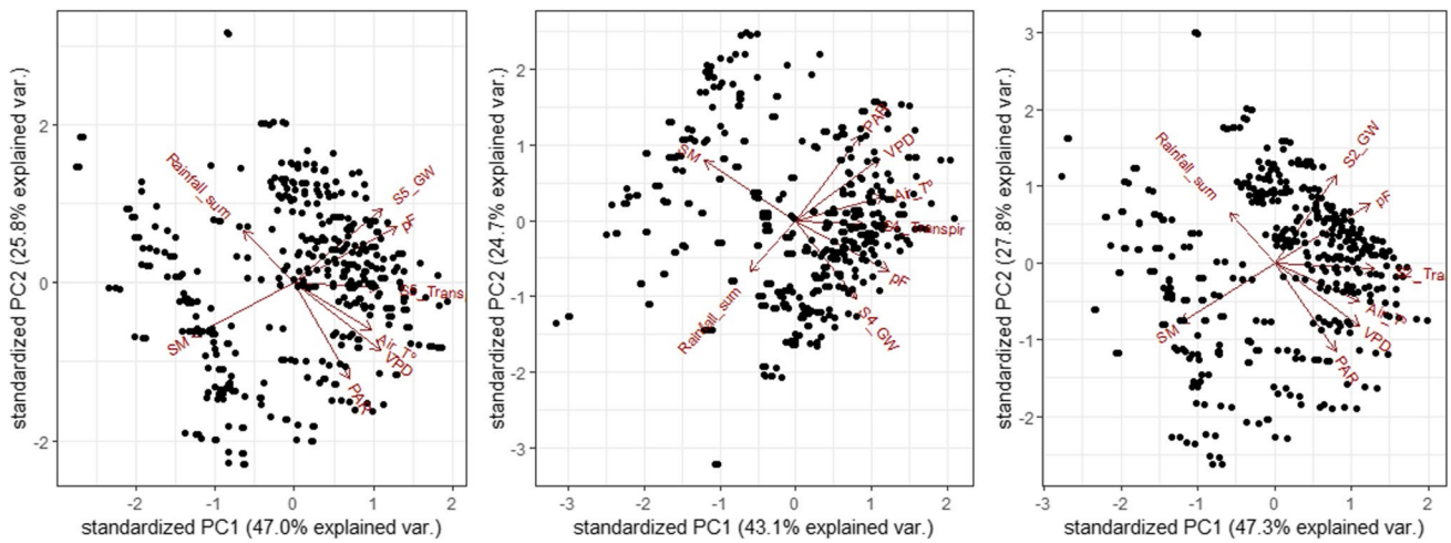
Fig. 7 Results of principal component analysis (PCA) for the site with higher groundwater level (S5-N, left), for the site with low groundwater level (S4-D, center), and for the site with fluctuating groundwater level (S2-F, right) including variance per principal components (PC) 1 and 2. Analyzed variables included daily mean groundwater level (GW), daily median of all the sensors of soil mois-
