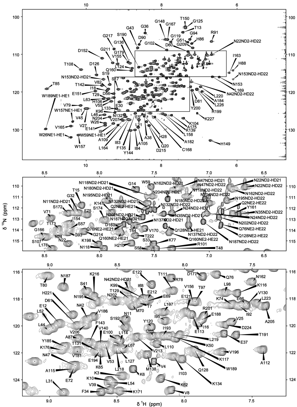
Fig. 1 ^1\text{H} - ^{15}\text{N} HSQC spectra of the BcII metallo- \beta -lactamase. The full spectrum is shown at the top , with crowded regions shown as expansions below. The resonance assignments of the backbone, side chain amide and tryptophan indole NH resonances are indicated
