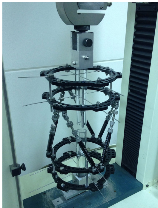
Fig. 2 A fine-wire Taylor Spatial Frame™ mounted in the axial testing apparatus (Tinius Olsen H25K-S UTM; Tinius Olsen Inc) is shown.
