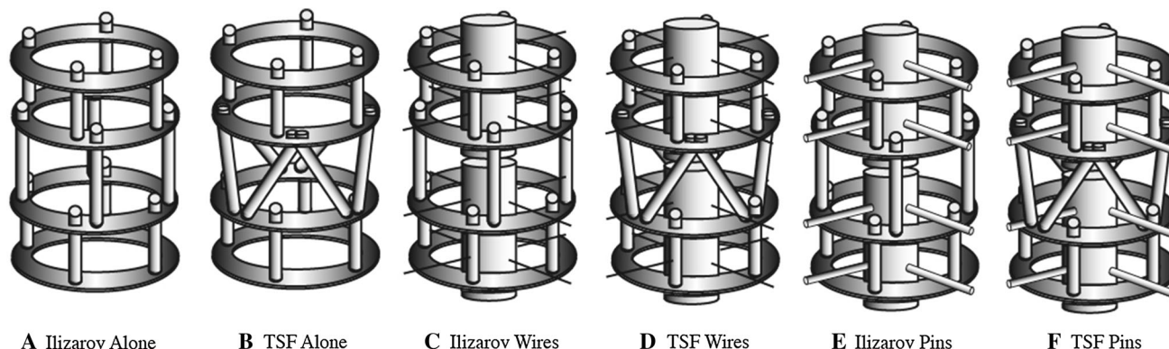
Fig. 1A–F The six frame constructs tested were the (A) Ilizarov alone, (B) Taylor Spatial Frame™ (TSF) alone, (C) fine-wire Ilizarov, (D) fine-wire TSF, (E) half-pin Ilizarov, and (F) half-pin TSF.
