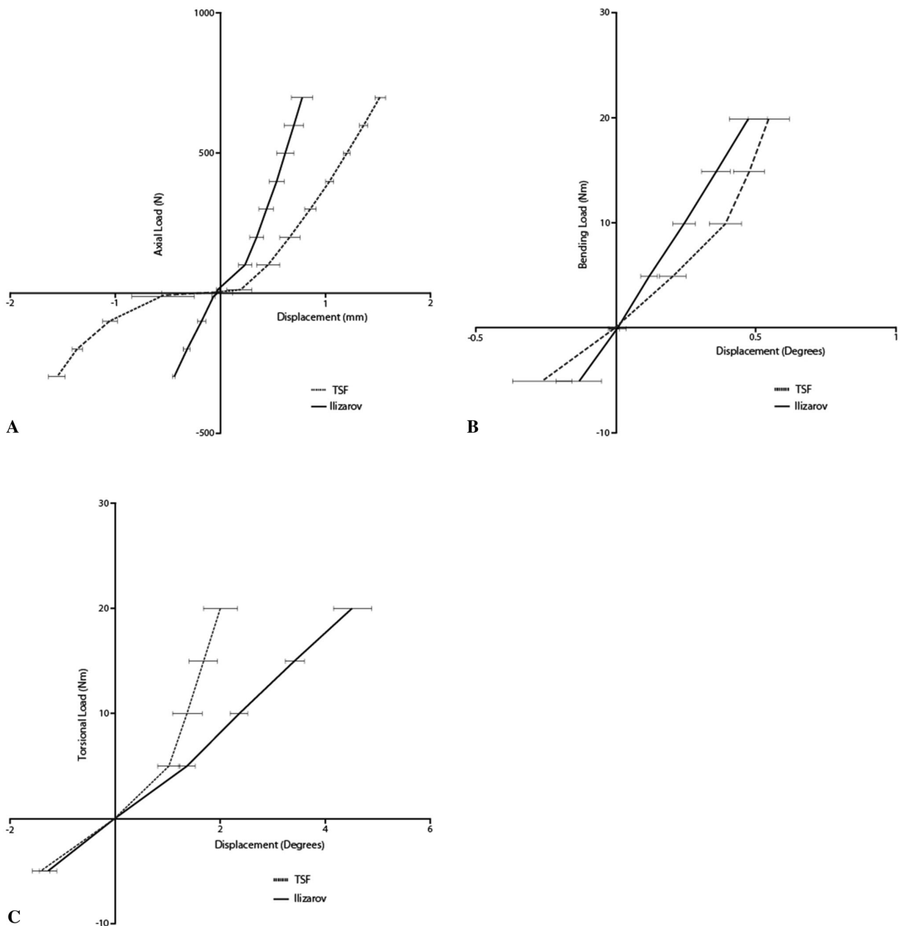
Fig. 3A–C Load deformation plots for testing of frame elements alone under (A) axial, (B) bending, and (C) torsional loads are shown. TSF = Taylor Spatial Frame™.
