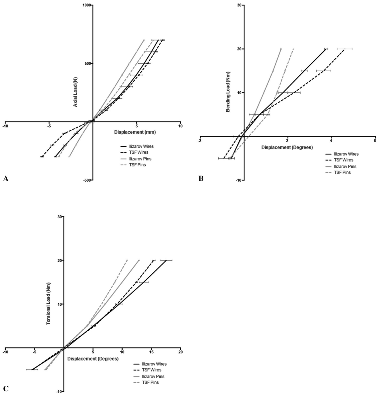
Fig. 5A–C Load deformation plots for testing of bone-frame constructs under (A) axial, (B) bending, and (C) torsional loads are shown. TSF = Taylor Spatial Frame™.
