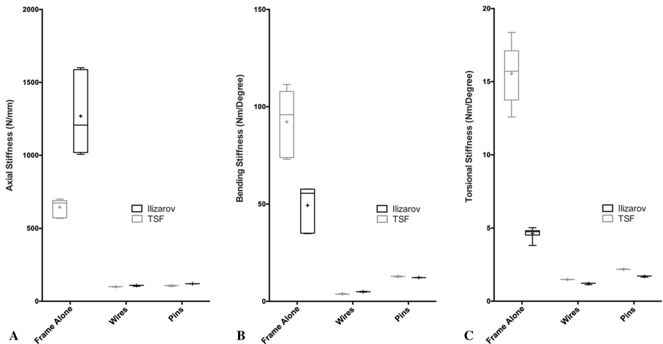
Fig. 4A–C Box and whisker plots of stiffness data for Ilizarov and TSF elements alone, fine-wire, and half-pin constructs under (A) axial, (B) bending, and (C) torsional loading are shown. The boxes
