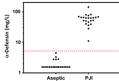
Fig. 1 \alpha -Defensin concentrations in patients with aseptic disease versus PJI are demonstrated. Note that concentrations are depicted on a log scale.
