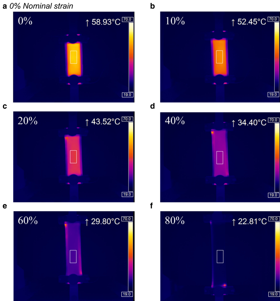
Fig. 3: The effect of nominal strain on the temperature output of the 15 × 5 cm printed stretchable carbon heaters at 15 V in a 19°C environment while at nominal strains; (a) 0% nominal strain, (b) 10% nominal strain, (c) 20% nominal strain, (d) 40% nominal strain, (e) 60% nominal strain, (f) 80% nominal strain
