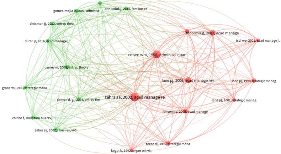
Fig.3 Co-citation analysis
