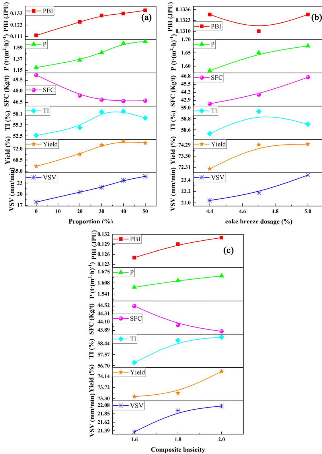
Fig. 2. Effect of process conditions on the agglomeration indexes of CAP (a) pelletized feed proportion, (b) coke breeze dosage, (c) composite.
