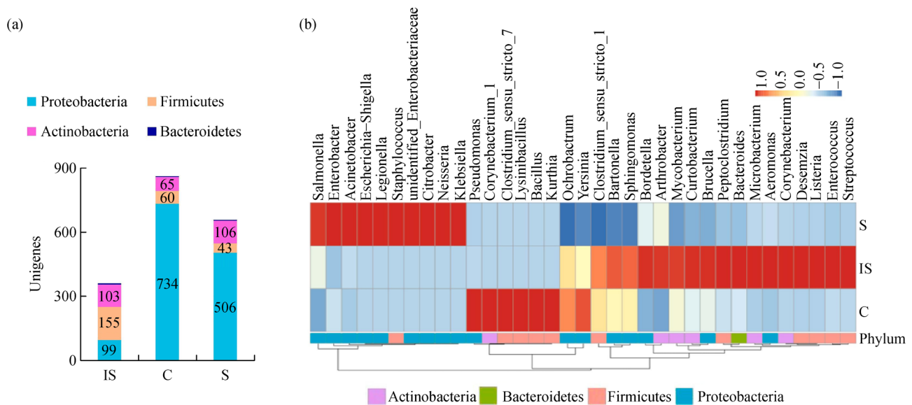
Fig. 2 Unigenes of human pathogenic bacteria at the phylum level (a) and their relative abundances (log 10 -transformed) at the genus level (b) in different samples obtained from initial sludge (IS), control (C), and sludge vermicompost (S). Reprinted with permission from Elsevier (Huang et al., 2020).
