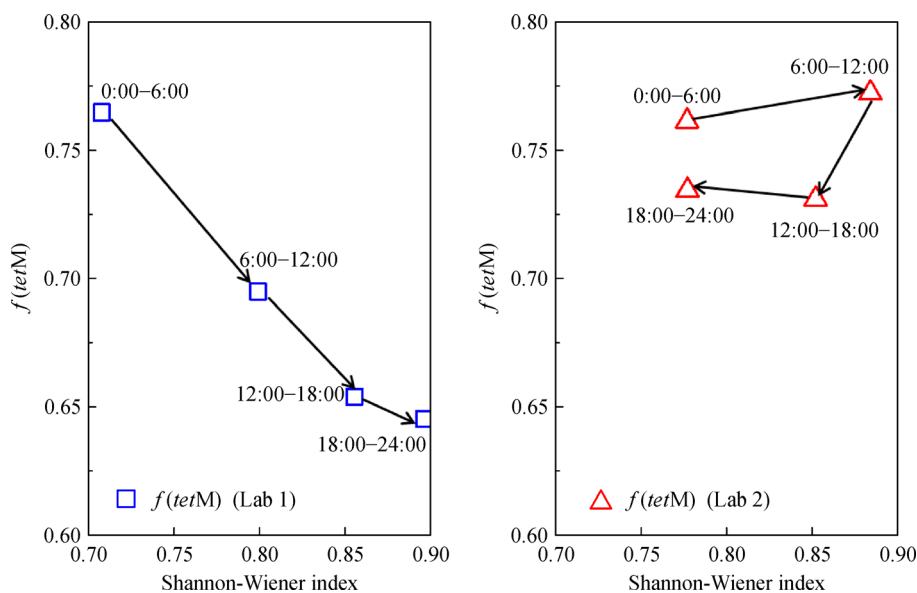
Fig. 8 Temporal variation of tetM abundance in the two laboratories.
