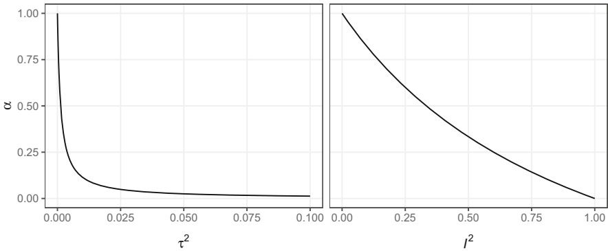
Fig. 4 The heterogeneity \tau^2 and relative heterogeneity I^2 = \tau^2/(\tau^2 + \sigma_o^2) of a hierarchical model versus the power parameter \alpha from a power prior model which lead to matching posteriors for the effect sizes \theta and \theta_r . The variance of the original effect estimate \sigma_o^2 = 0.05^2 from the “Labels” experiment is used for the transformation to the heterogeneity scale \tau^2
