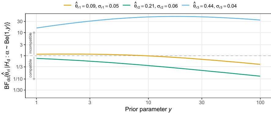
Fig. 2 Sensitivity of the Bayes factor \text{BF}_{\text{dc}}\{\hat{\theta}_r | \mathcal{H}_d : \alpha \sim \text{Be}(1, y)\} with respect to the parameter y of the partial discounting prior under \mathcal{H}_d
