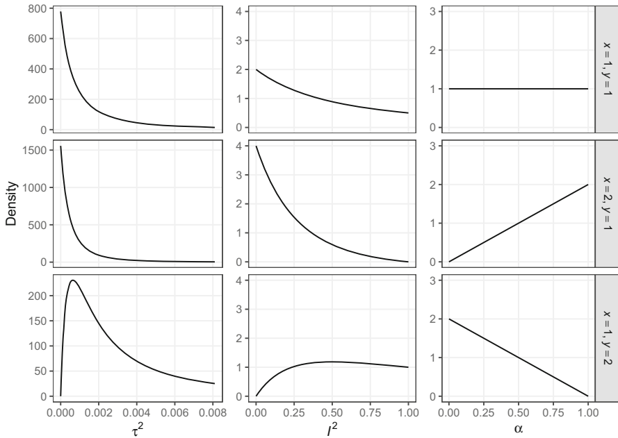
Fig. 5 Priors on the heterogeneity \tau^2 \sim \text{GF}(y, x, 2/\sigma_o^2) (left), the relative heterogeneity I^2 = \tau^2/(\sigma_o^2 + \tau^2) \sim \text{GBe}(y, x, 2) (middle) and the power parameter \alpha \sim \text{Be}(x, y) (right) that lead to matching marginal posteriors for effect sizes \theta and \theta_r . The variance of the original effect estimate \sigma_o^2 = 0.05^2 from the “Labels” experiment is used for the transformation to the heterogeneity scale \tau^2
