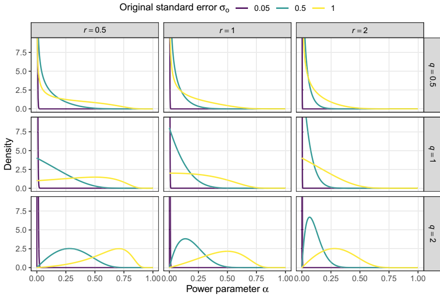
Fig. 6 Prior for the power parameter \alpha implied by an inverse gamma prior \mathcal{H}_d: \tau^2 \sim \text{IG}(q, r) in a hierarchical model with consistent test for \mathcal{H}_c: \tau^2 = 0 versus \mathcal{H}_d: \tau^2 > 0
