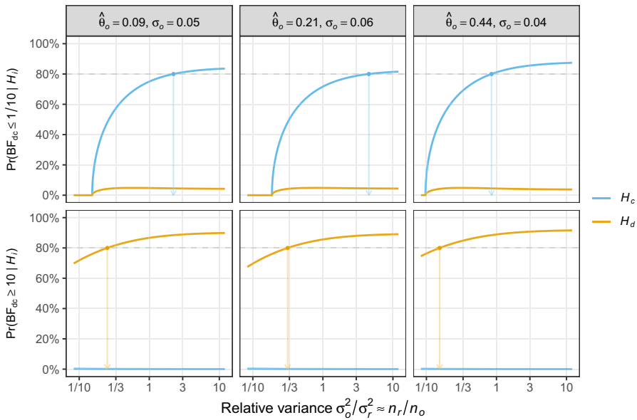
Fig. 3 Probability of replication success as a function of relative variance for the three replications of experiment “Labels” regarded as original study. The arrows point to the relative variance associated with an 80% probability under the respective hypotheses
