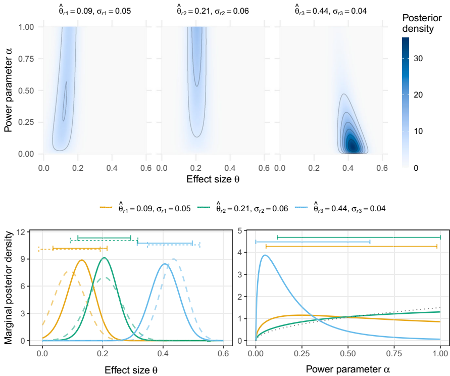
Fig. 1 Joint (top) and marginal (bottom) posterior distributions of effect size \theta and power parameter \alpha based on data from the “Labels” experiment (Protzko et al. 2020). The dashed lines depict the posterior density for the effect size \theta when the replication data are analyzed in isolation without incorporation of the original data. The horizontal error bars represent the corresponding 95% highest posterior density credible intervals. The dotted line represents the limiting posterior density of the power parameter \alpha for perfectly agreeing original and replication studies
