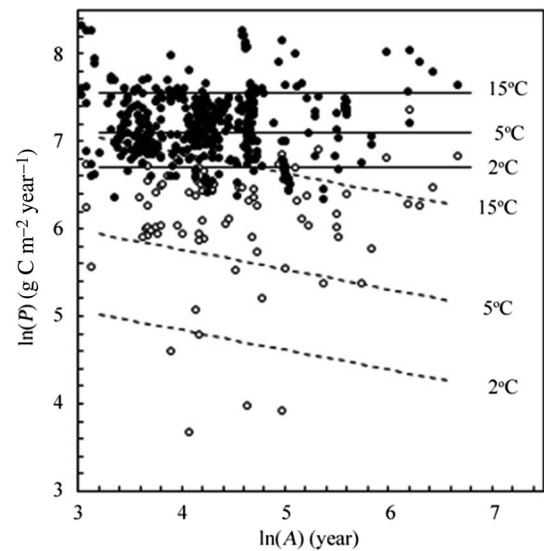
Fig. 2 Scatter plots of the natural logarithm [ln()] of GPP (filled circle) and NPP (open circle) against the natural logarithm of forest age for the data used here. The solid lines show how predicted values of GPP vary with age at sites with each of three mean annual temperatures as determined using Eq. (4). The dashed lines show similar predictions of NPP using Eq. (5). P was productivity (GPP or NPP, g C m -2 year -1 ), and A was forest age (year)
