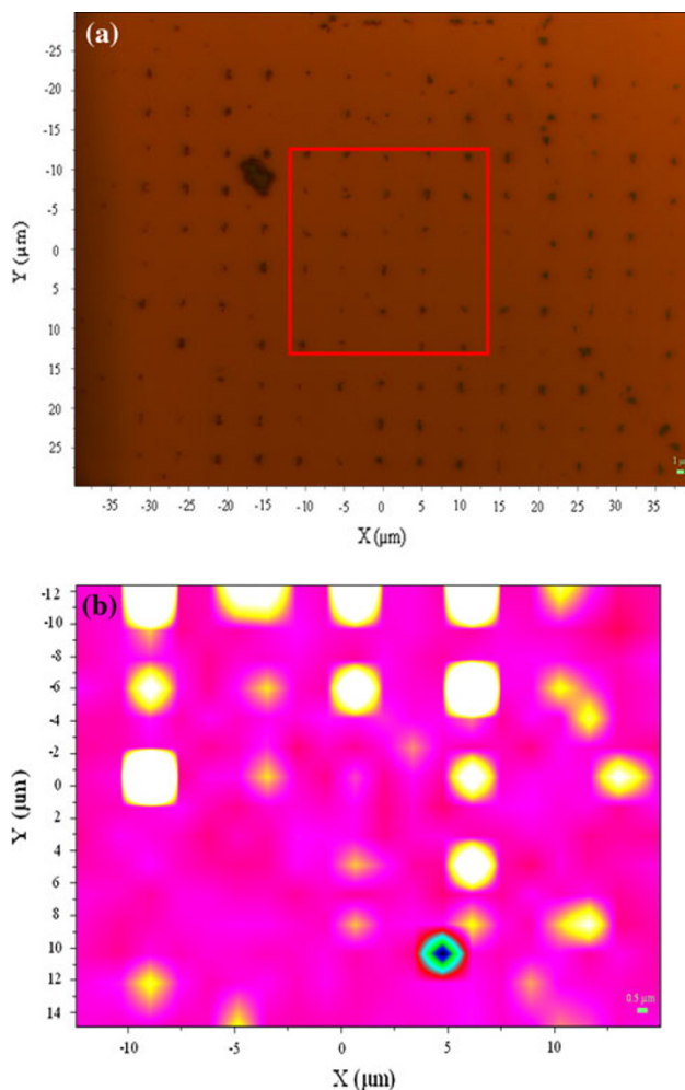
Fig. 5 a Optical image of the 2D mapping area, indicated by the square and b image of the 2D Raman intensity mapping
